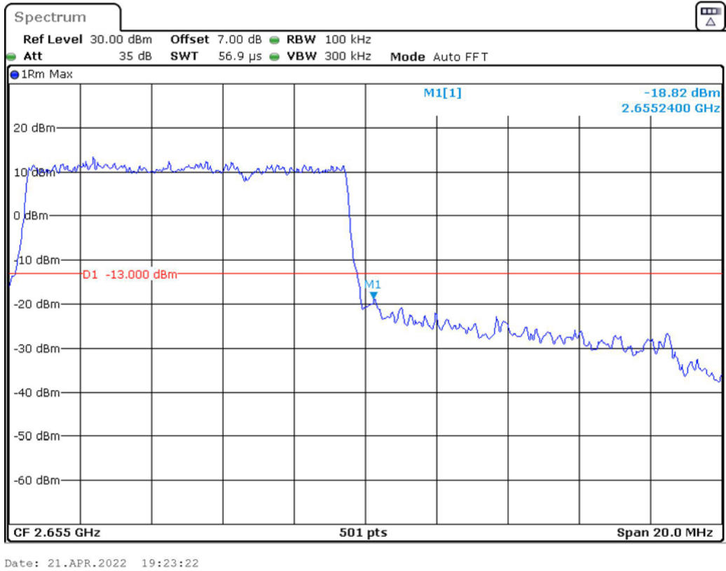
Band 41_10 MHz_High_QPSK_RB50#0
