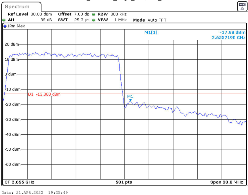
Band 41_15 MHz_High_16QAM_RB75#0
