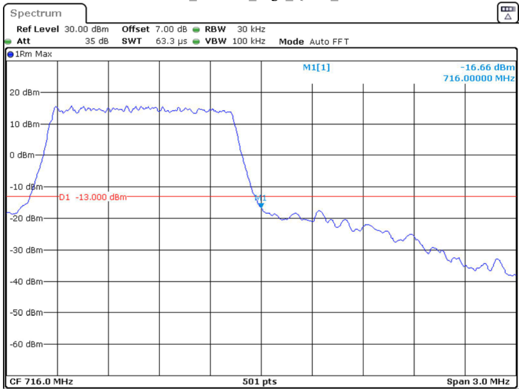
Band 12_1.4 MHz_High_QPSK_RB6#0
