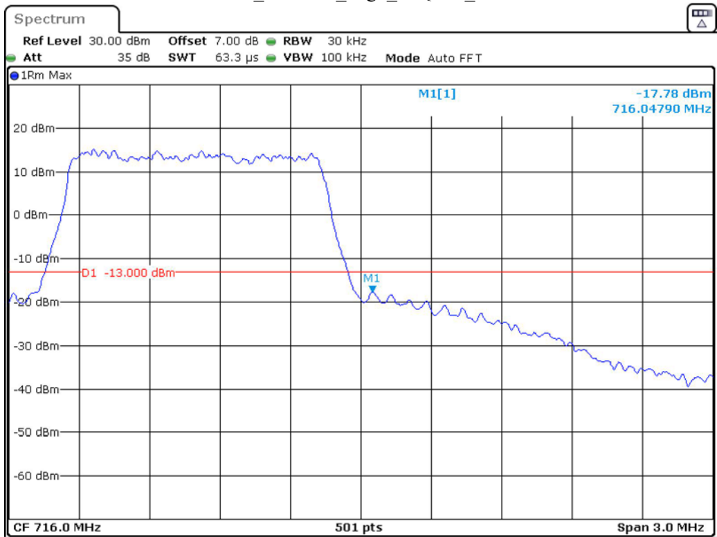
Band 12_1.4 MHz_High_16QAM_RB6#0
