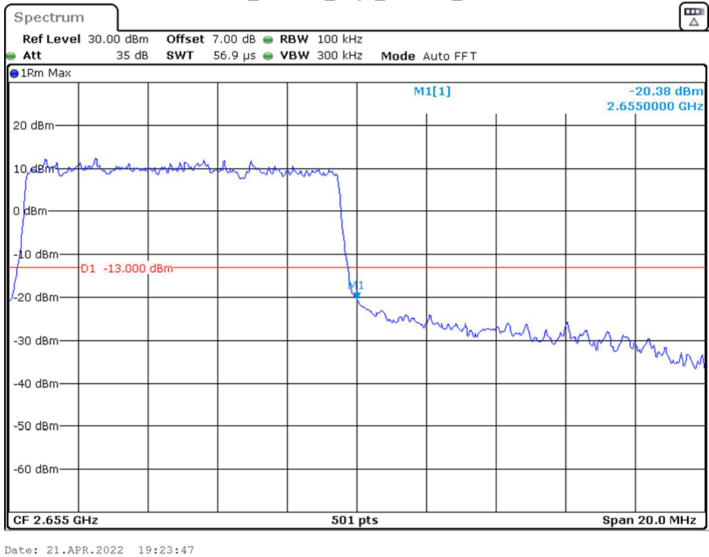
Band 41_10 MHz_High_16QAM_RB50#0
