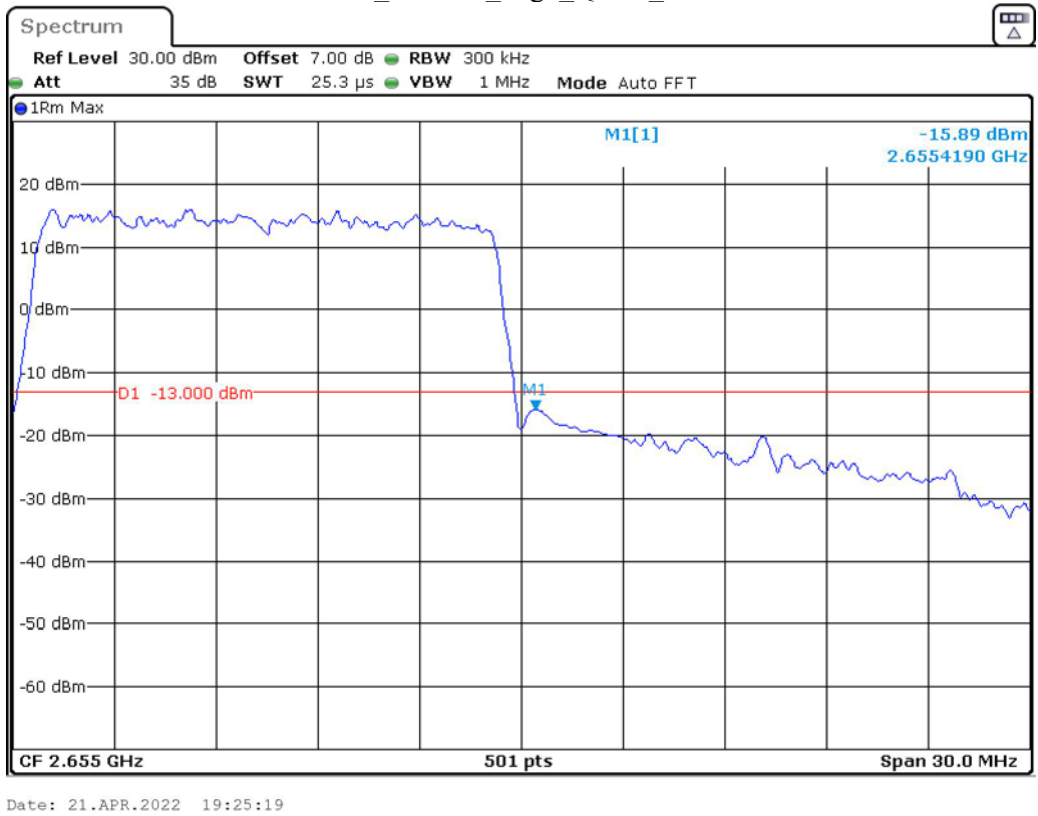
Band 41_15 MHz_High_QPSK_RB75#0
