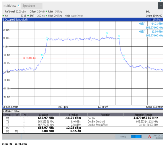
1-N71--15-5-L-3-DFT-16QAM-Outter_Full-25@0-Ant1- 4.479-5.080-≤5-PASS
