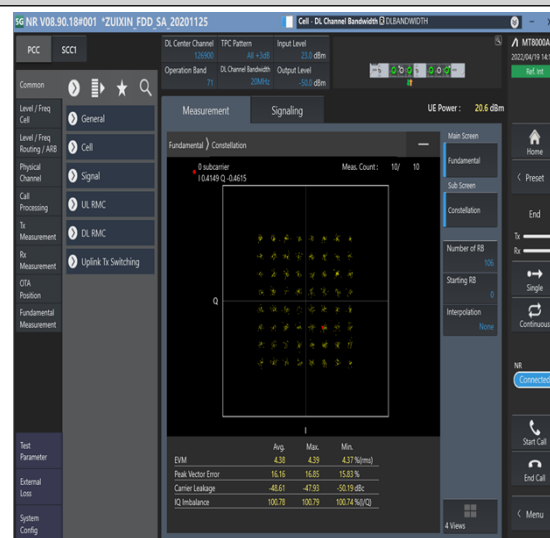
1-N71--15-20-M-8-CP-64QAM-Outer_Full-106@0-Ant1-see graph-PASS
