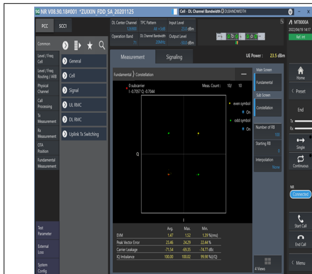
1-N71--15-20-M-1-DFT-PI2BPSK-Outer_Full-100@0-Ant1-see graph-PASS
