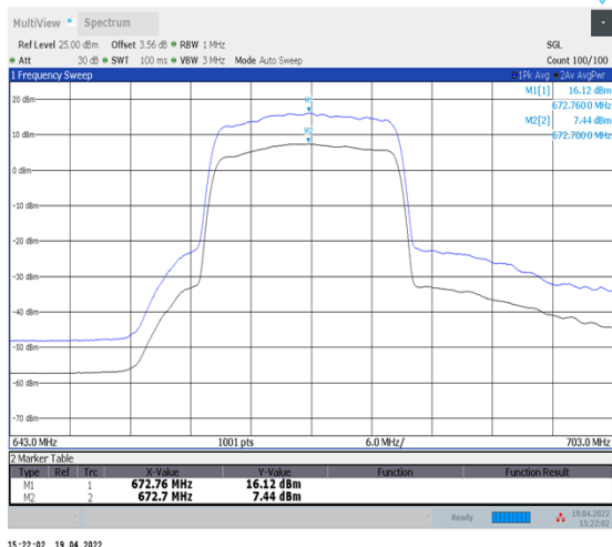
1-N71--15-20-L-1-DFT-256QAM-Outer_Full-100@0- Ant1-8.68-100%-0.00-8.68-PASS-≤13
