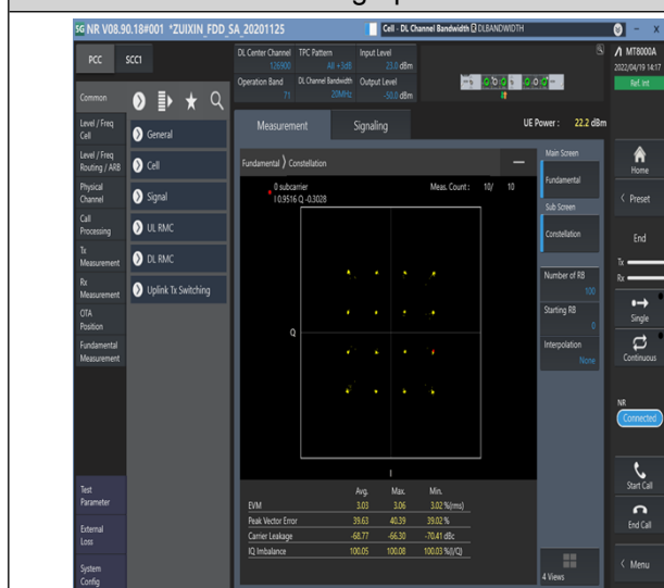
1-N71--15-20-M-3-DFT-16QAM-Outer_Full-100@0-Ant1-see graph-PASS
