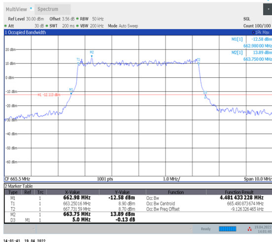
1-N71--15-5-L-1-DFT-QPSK-Outter_Full-25@0-Ant1- 4.481-5.000-≤5-PASS
