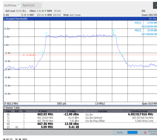
1-N71--15-5-L-2-DFT-PI2BPSK-Outter_Full-25@0-Ant1- 4.502-5.090-≤5-PASS
