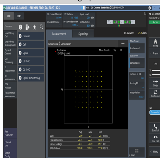
1-N71--15-20-M-4-DFT-64QAM-Outer_Full-100@0-Ant1-see graph-PASS
