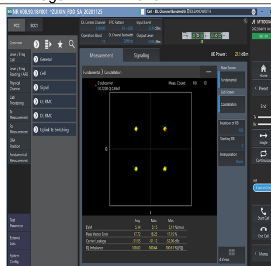
1-N71--15-20-M-6-CP-QPSK-Outer_Full-106@0-Ant1-see graph-PASS
