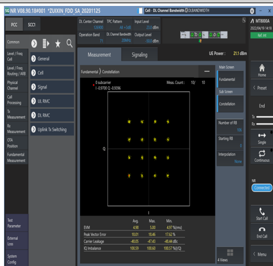
1-N71--15-20-M-7-CP-16QAM-Outer_Full-106@0-Ant1-see graph-PASS
