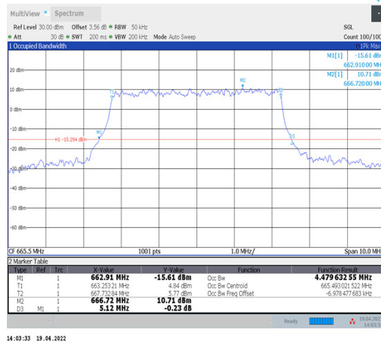
1-N71--15-5-L-4-DFT-64QAM-Outter_Full-25@0-Ant1- 4.48-5.120-≤5-PASS
