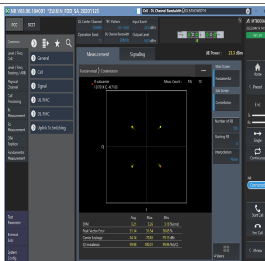
1-N71--15-20-M-2-DFT-QPSK-Outer_Full-100@0-Ant1-see graph-PASS
