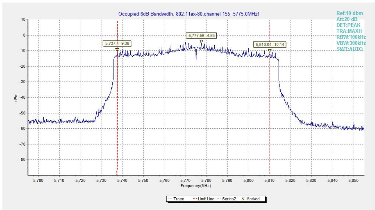
Fig. 26 Occupied 6dB Bandwidth (802.11ax-HE80, 5775MHz)
