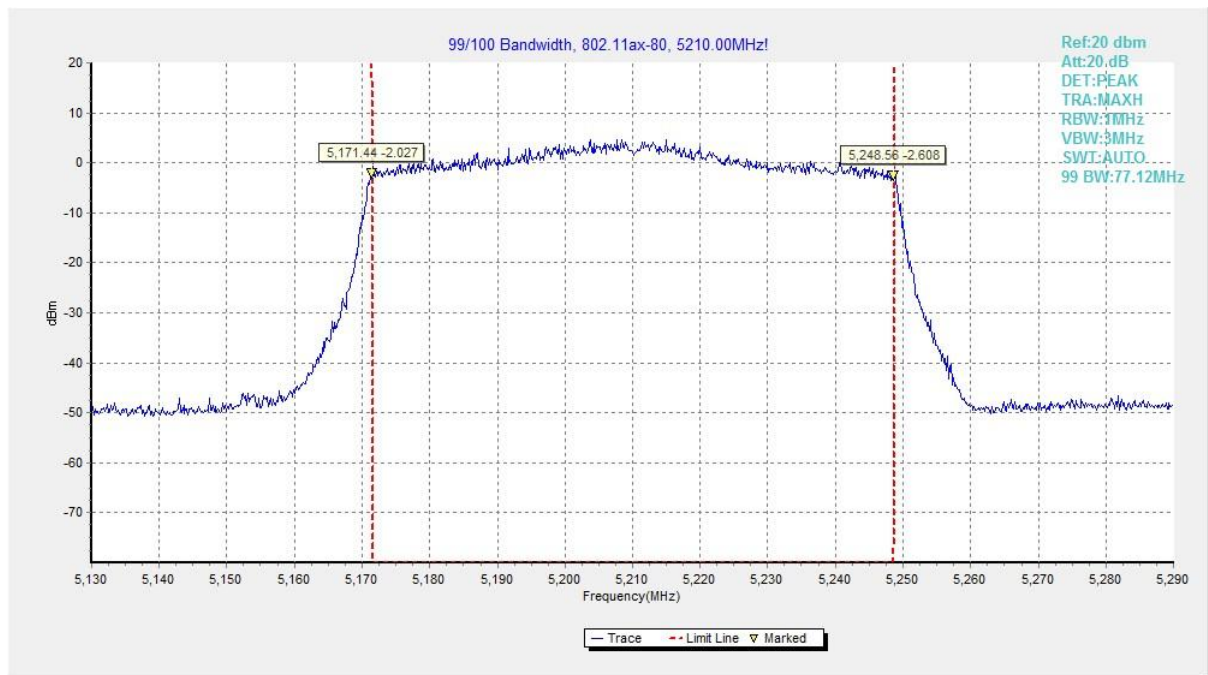
Fig. 47 99% Occupied Bandwidth (802. 11ax-HE80, 5210MHz)
