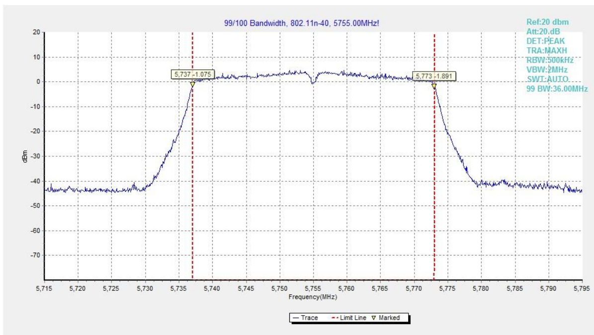
Fig. 45 99% Occupied Bandwidth (802.11n-HT40, 5755MHz)
