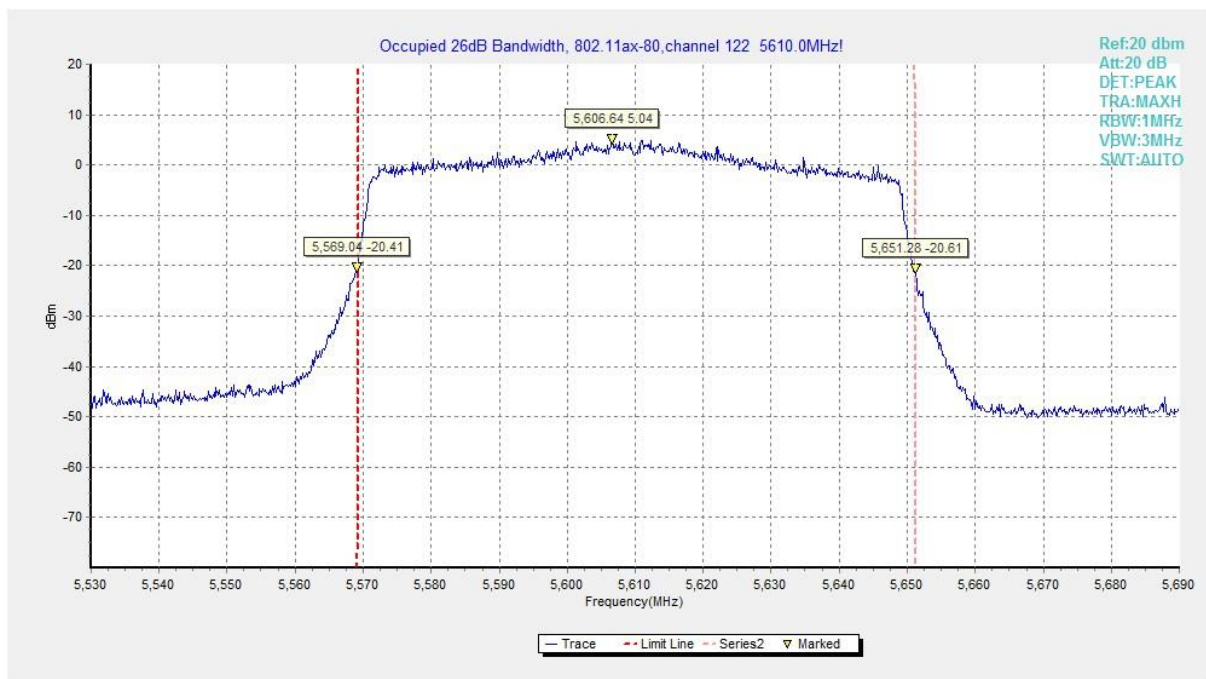
Fig. 18 Occupied 26dB Bandwidth (802. 11ax-HE80, 5610MHz)
