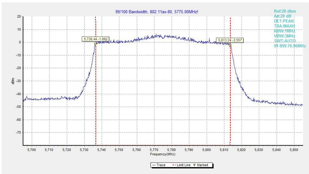
Fig. 50 99% Occupied Bandwidth (802. 11ax-HE80, 5775MHz)
