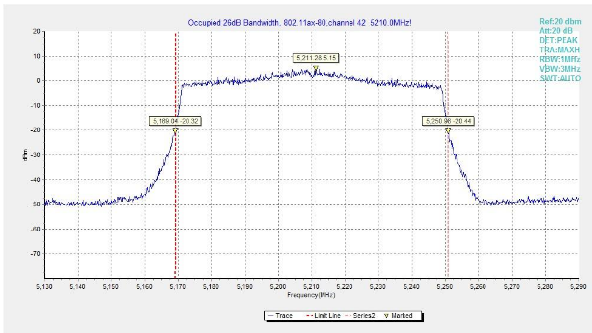
Fig. 16 Occupied 26dB Bandwidth (802.11ax-HE80, 5210MHz)
