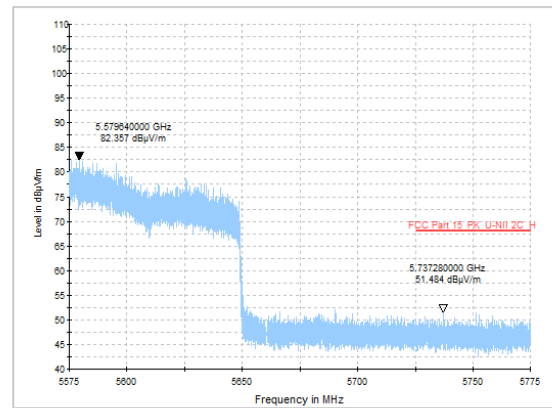
Fig. 70 Band Edges (802.11ax-HE160, CH114 5570MHz)
