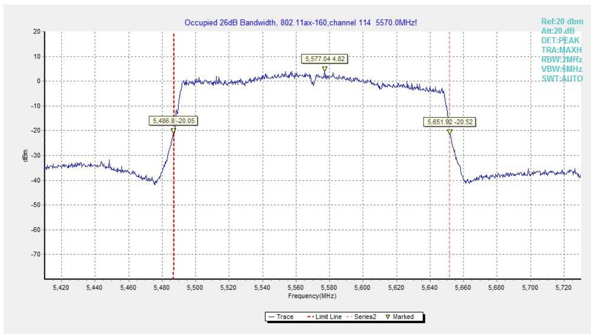
Fig. 20 Occupied 26dB Bandwidth (802. 11ax-HE160, 5570MHz)
