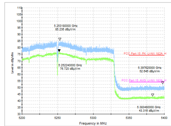
Fig. 69 Band Edges (802.11ax-HE160, CH50 5250MHz)
