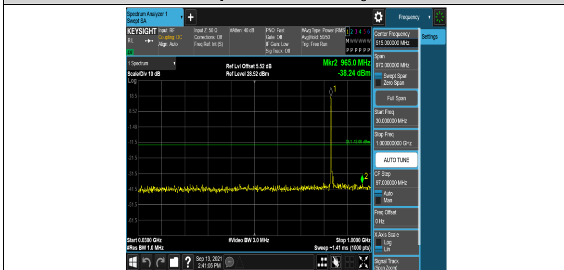
Band26-5MHz-16QAM-26915-1RB#0-Range3:30~1000MHz
