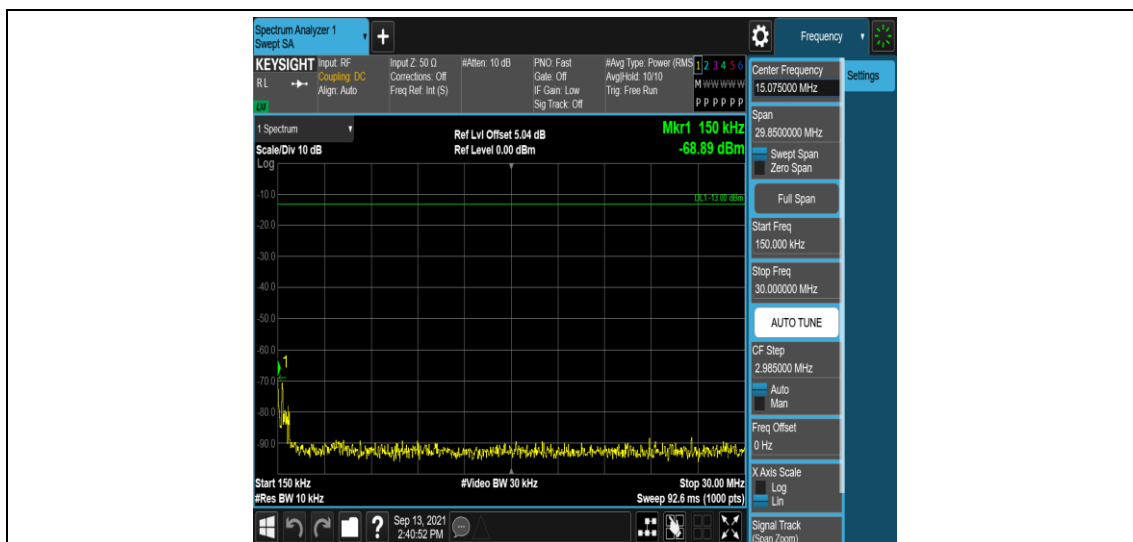
Band26-5MHz-16QAM-26915-1RB#0-Range2:0.15~30MHz
