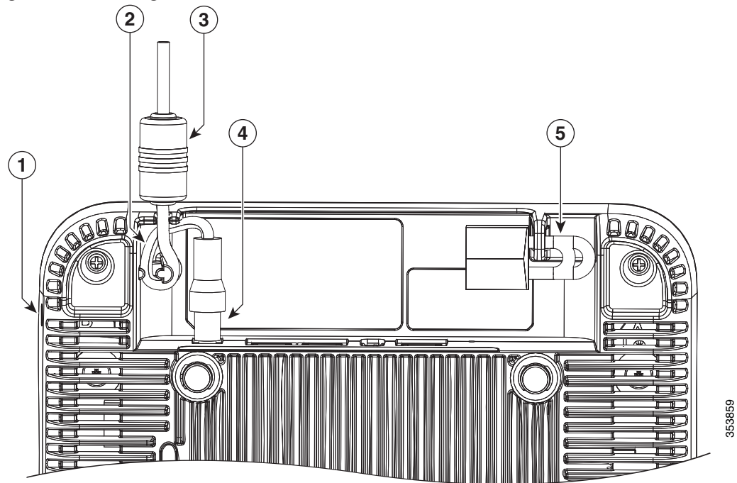
Figure 4 Routing the DC Power Cable
