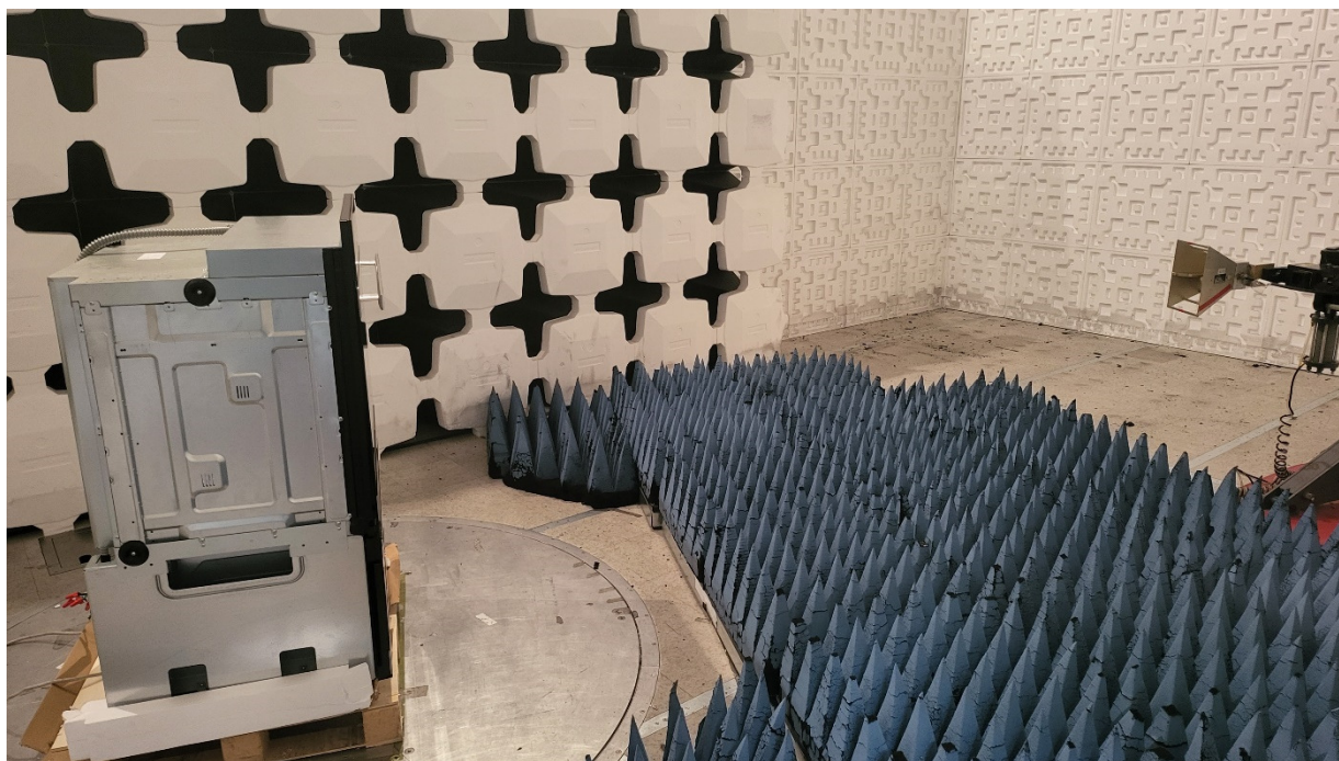
Figure 4. Radiated Emissions Measurement, above 1000 MHz and Variation in Operating Frequency
