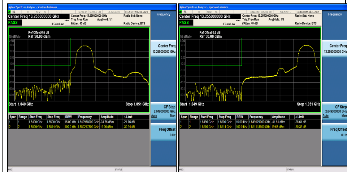
Band2_1.4MHz_64QAM_18607_1RB#0
