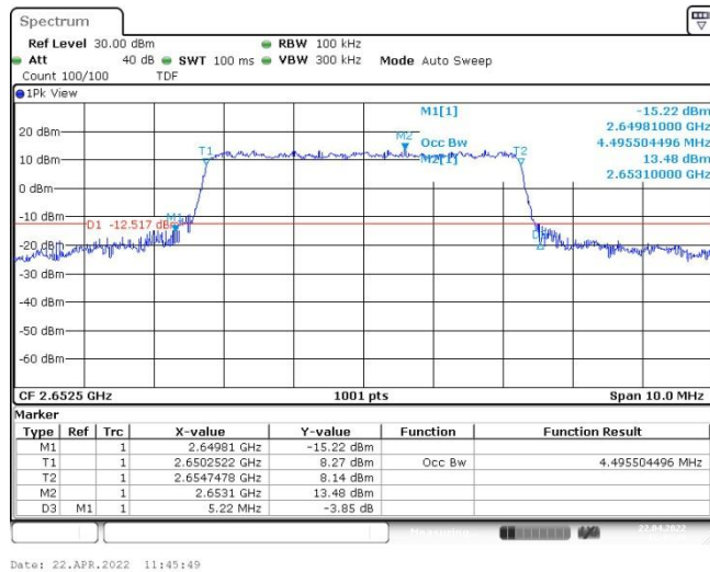
Band41-5MHz-16QAM-40265-25RB#0
