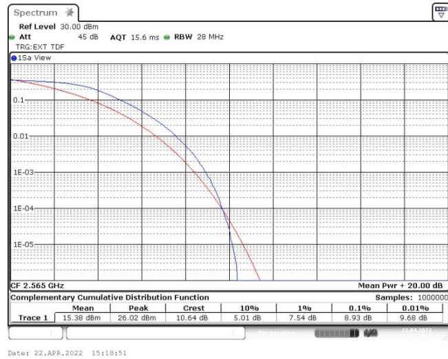
Band41-20MHz-QPSK-40620-100RB#0
