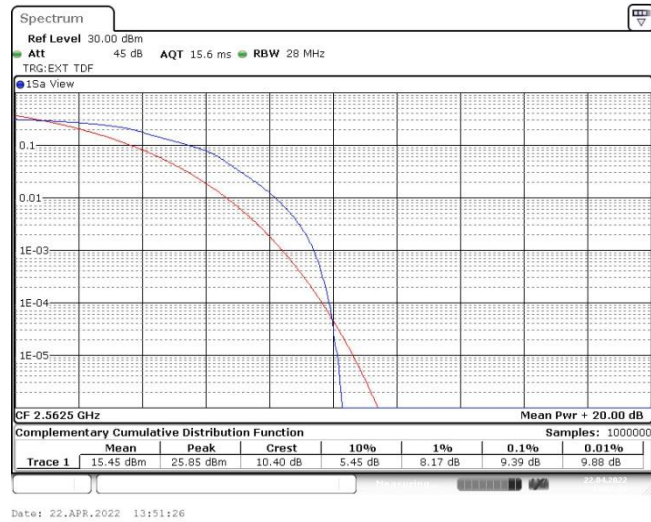
Band41-15MHz-16QAM-40620-75RB#0
