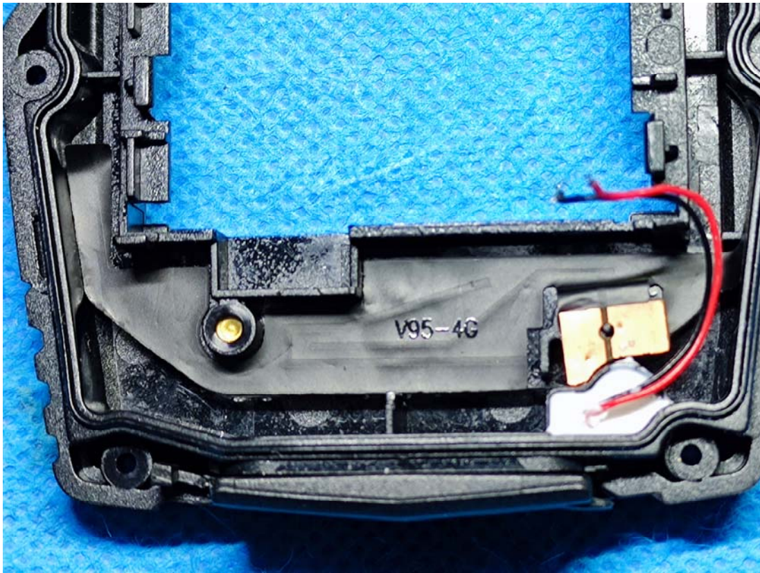
2G/3G Antenna
