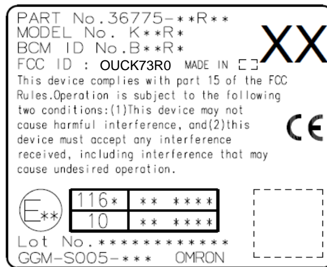
Figure 9.1 K73R0 Label
