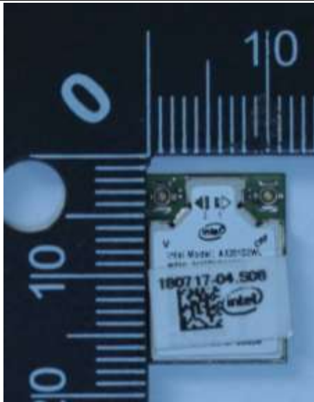
Adapter Front
