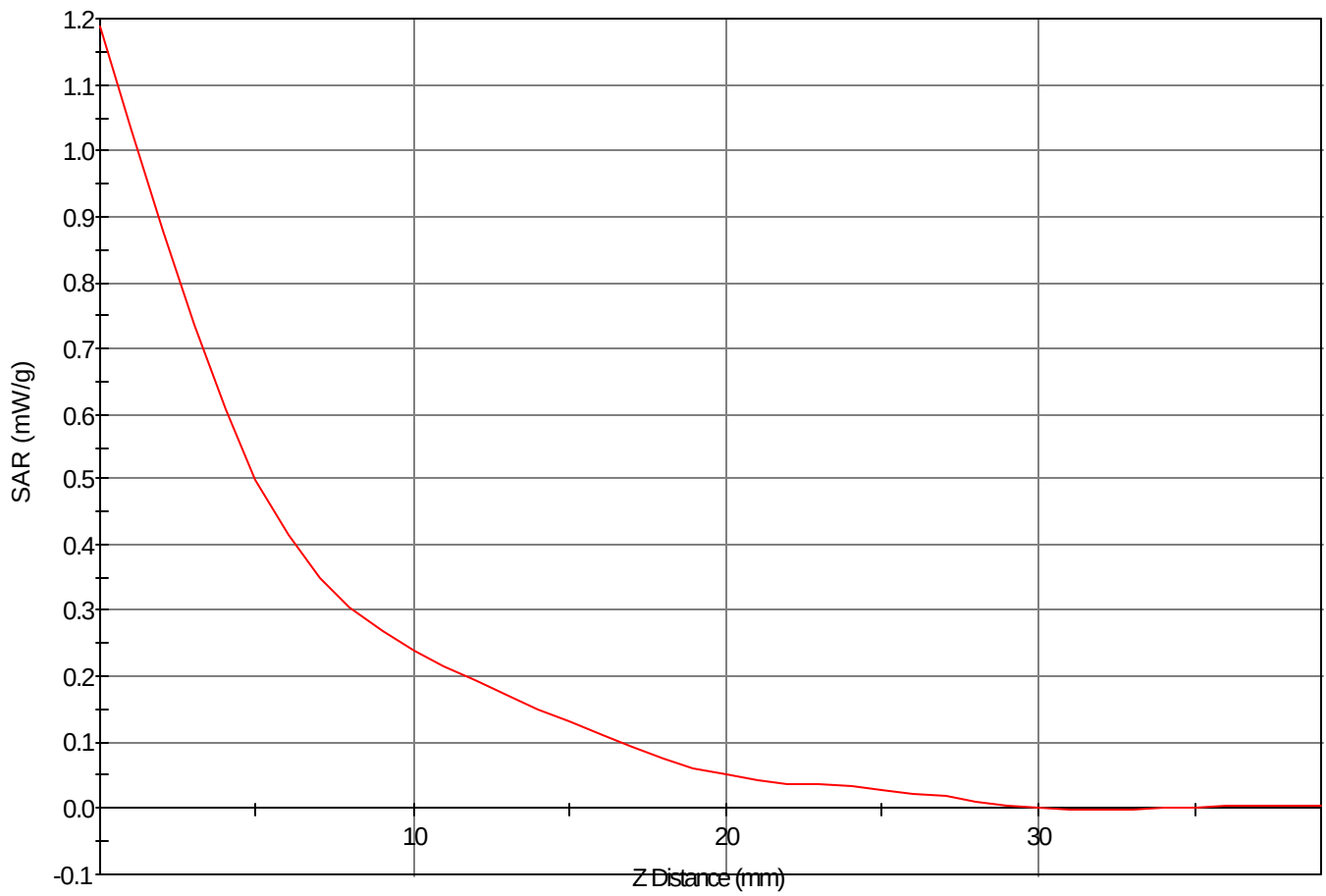
SAR - Z Axis at Hotspot x:-1.0 y:33.0
