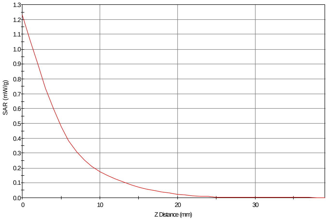
SAR - Z Axis at Hotspot x:-4.0 y:33.0
