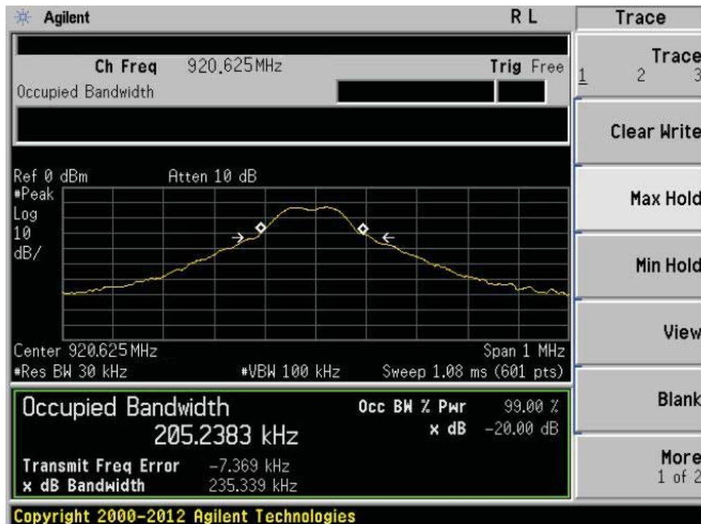
920.625MHz 20 dB Bandwidth
