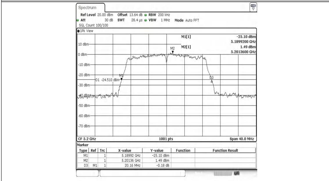
11AC20SISO-Ant1-5200
