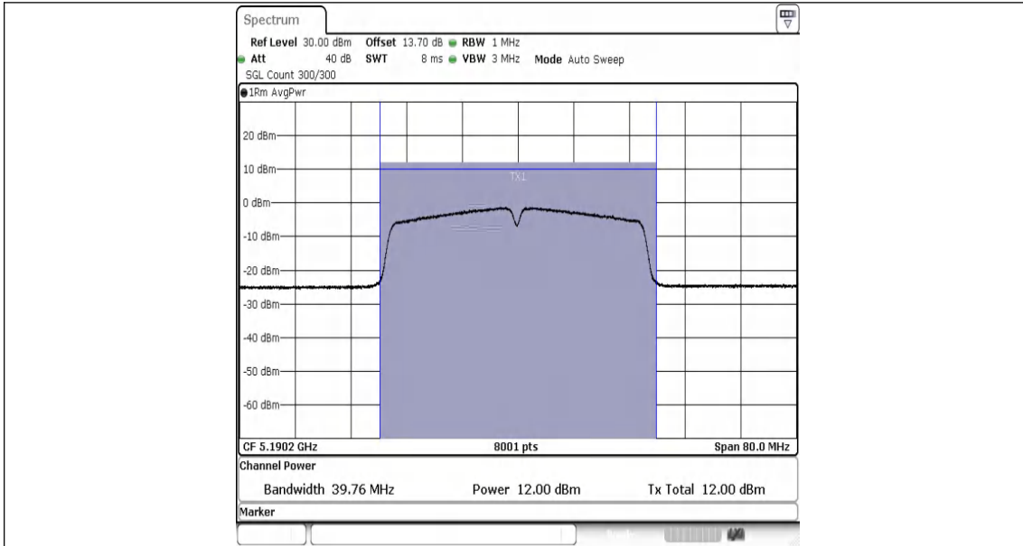
11AC40SISO-Ant1-5190-PASS
