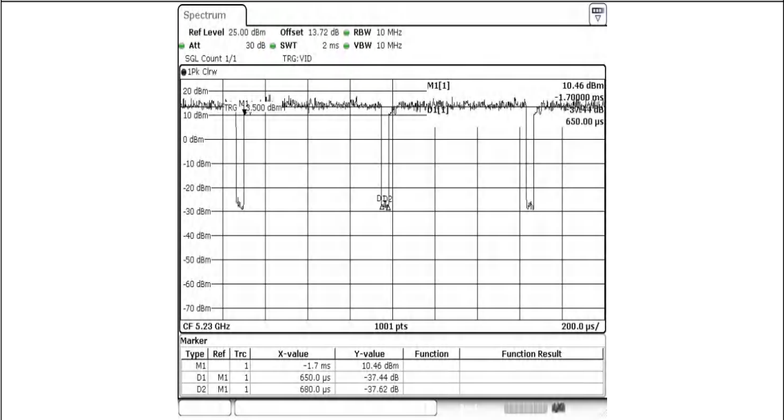
NTVN-11N40SISO-Ant1-5230
