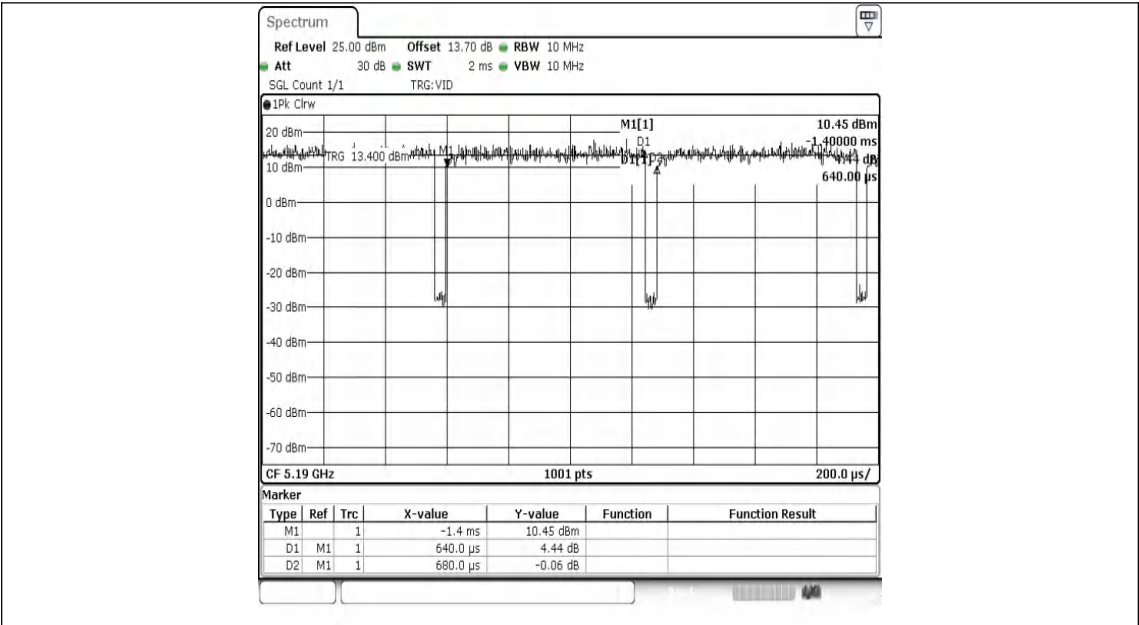
NTVN-11N40SISO-Ant1-5190
