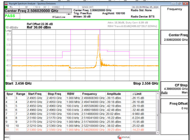
Band41 20MHz CP_OFDM_SCS30kHz QPSK RB51_0_CH501204
