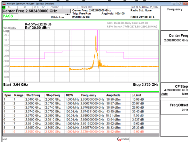
Band41_15MHz_CP_OFDM_SCS30kHz_QPSK_RB38_0_CH536496
