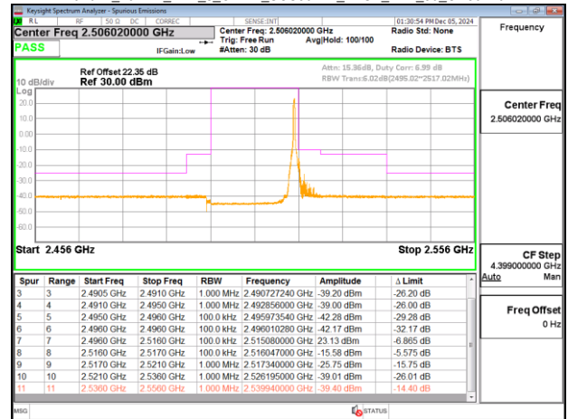
Band41_20MHz_DFT_s_OFDM_SCS30kHz_BPSK_RB50_0_CH501204
