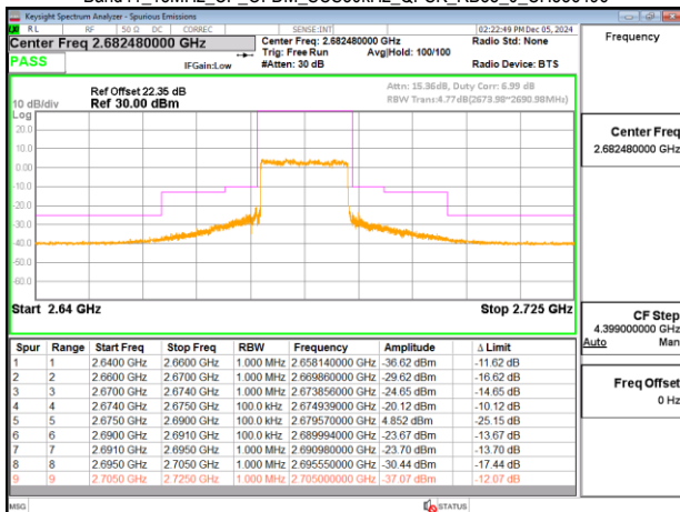
Band41_15MHz_CP_OFDM_SCS30kHz_QPSK_RB38_0_CH536496
