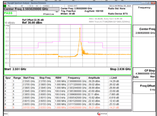
Band41_15MHz_DFT_s_OFDM_SCS30kHz_BPSK_RB36_0_CH518604
