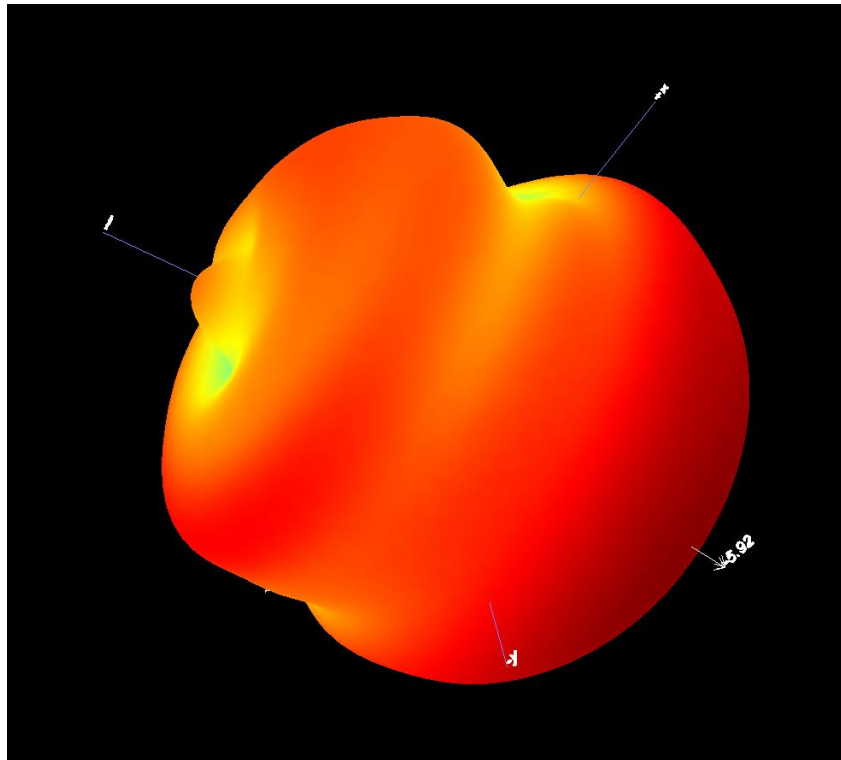
B1.3 3D Pattern for 2480MHz
