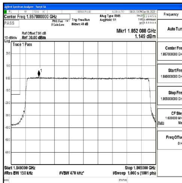
Band2_15MHz_16QAM_18675_75RB#0
