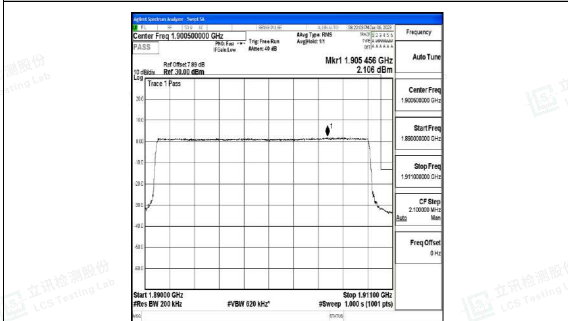
Band2_20MHz_16QAM_19100_100RB#0
