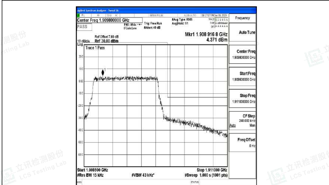
Band2_1.4MHz_16QAM_19193_6RB#0
