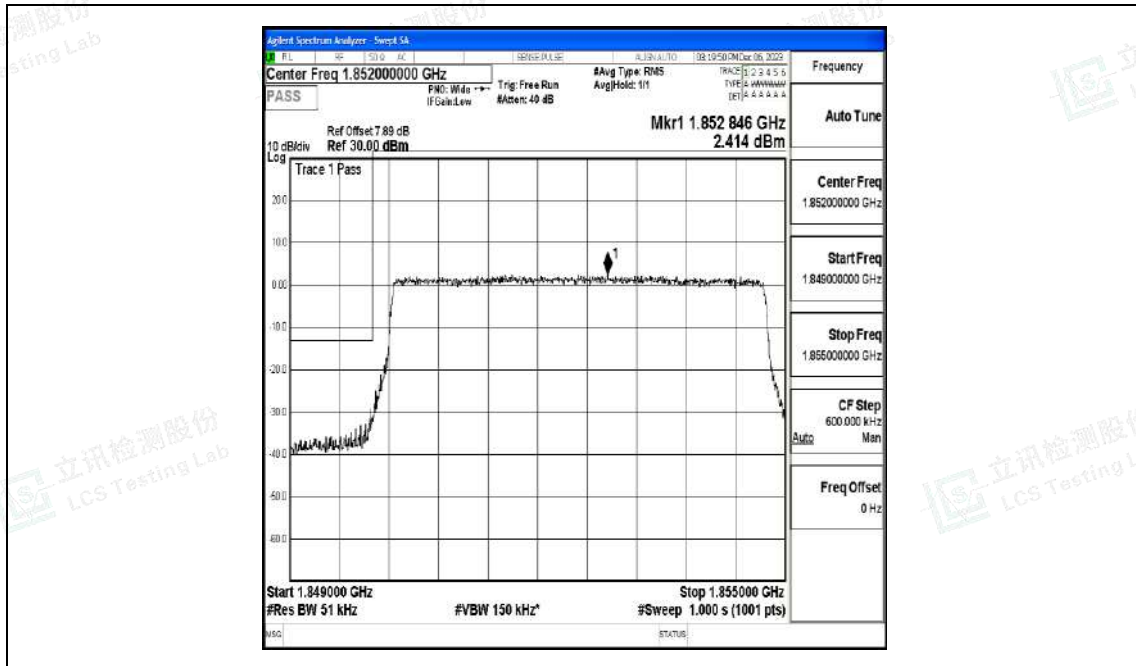
Band2_5MHz_QPSK_18625_25RB#0
