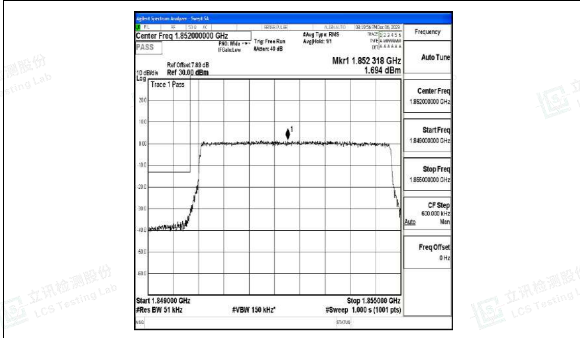
Band2_5MHz_16QAM_18625_25RB#0
