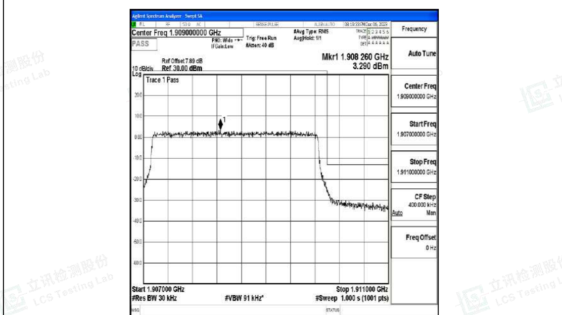
Band2_3MHz_16QAM_19185_15RB#0
