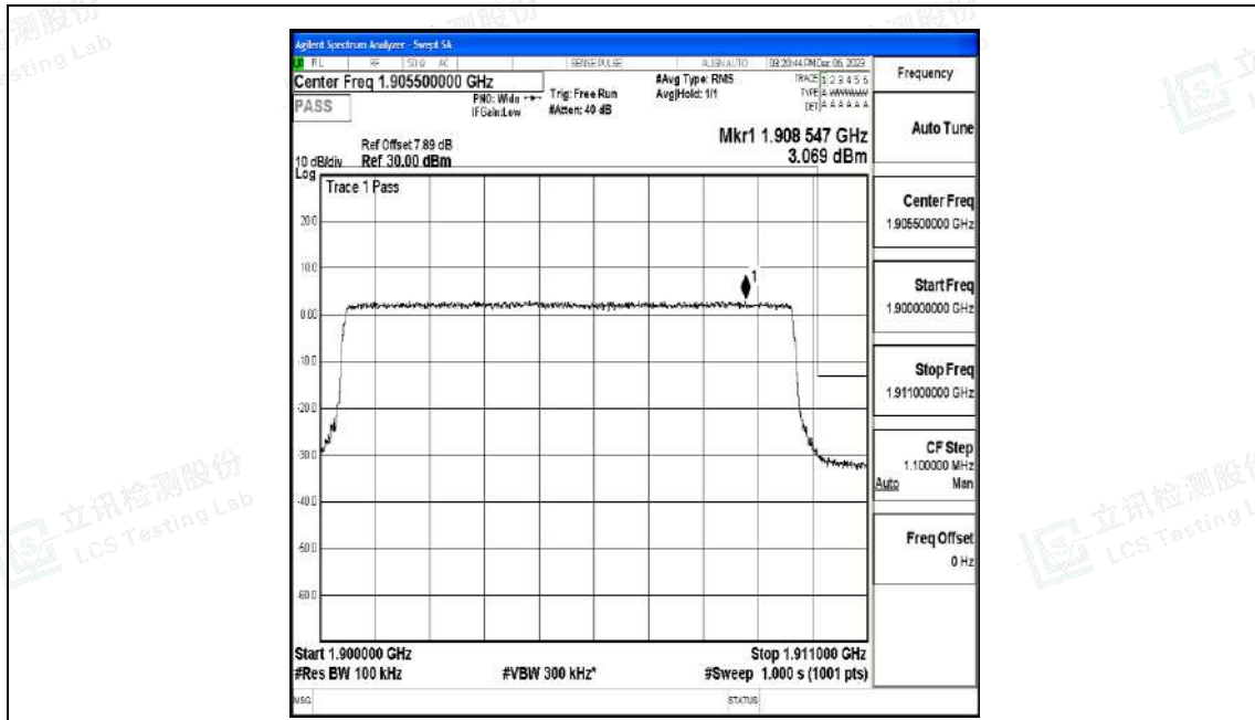
Band2_10MHz_QPSK_19150_50RB#0
