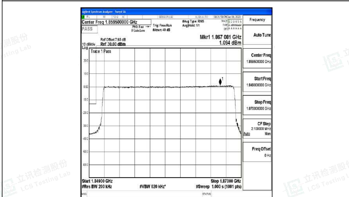
Band2_20MHz_16QAM_18700_100RB#0
