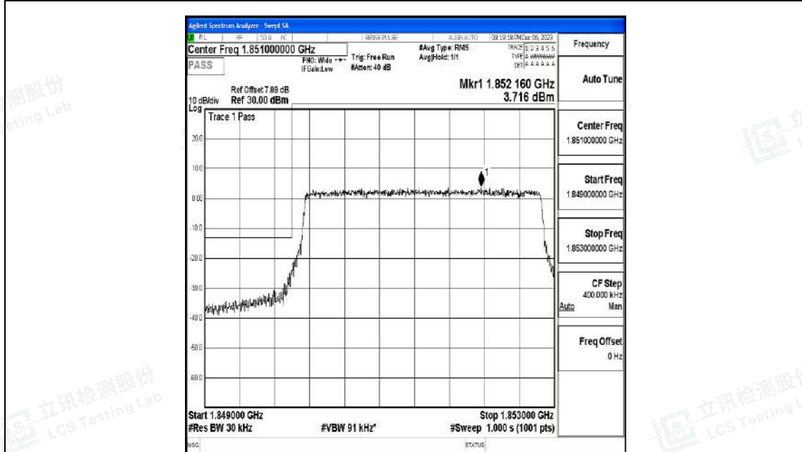
Band2_3MHz_16QAM_18615_15RB#0
