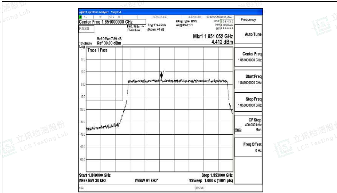
Band2_3MHz_QPSK_18615_15RB#0
