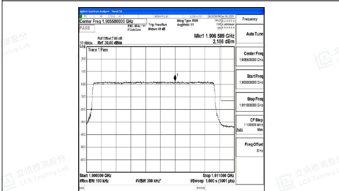
Band2_10MHz_16QAM_19150_50RB#0
