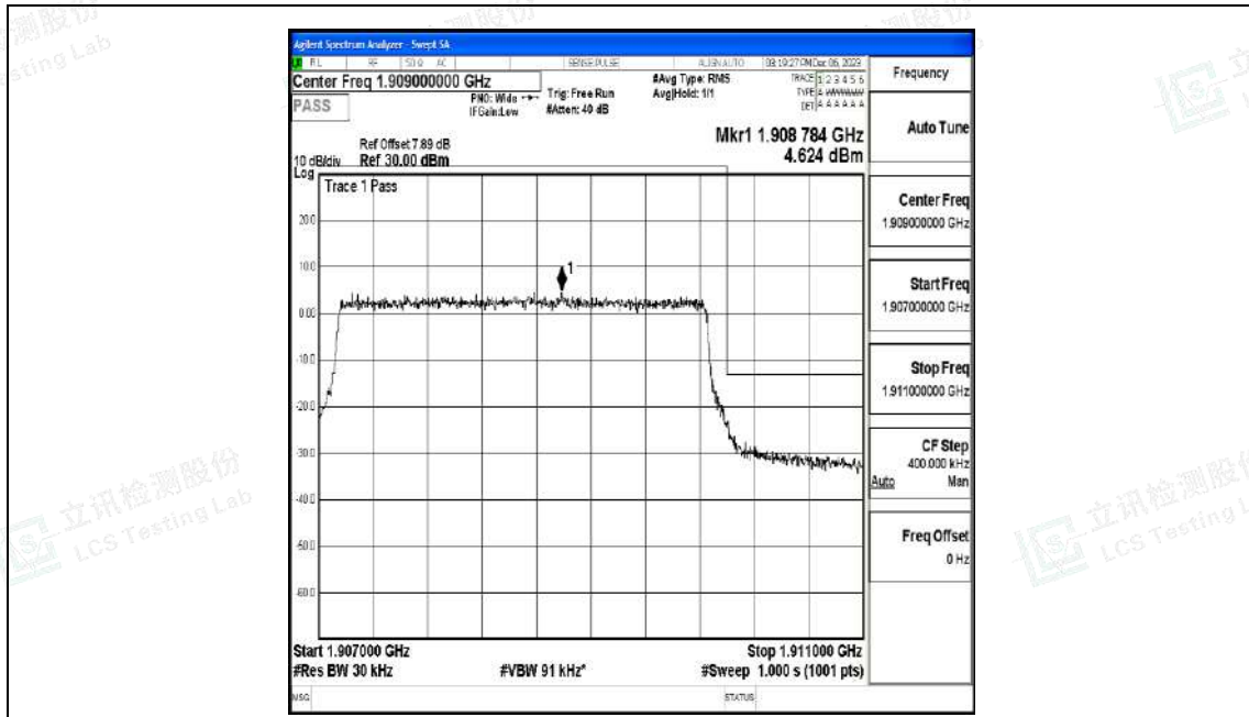
Band2_3MHz_QPSK_19185_15RB#0
