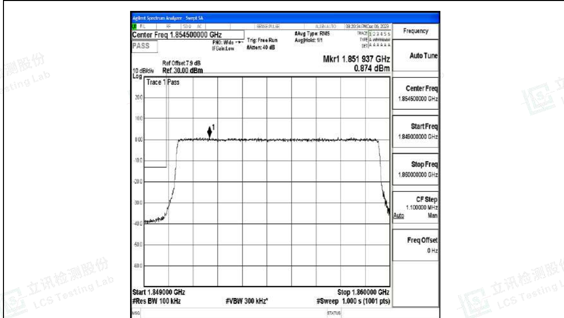
Band2_10MHz_16QAM_18650_50RB#0
