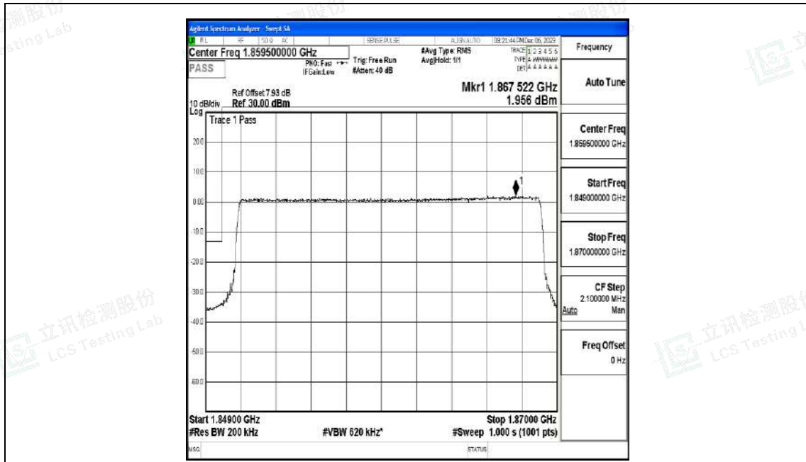
Band2_20MHz_QPSK_18700_100RB#0
