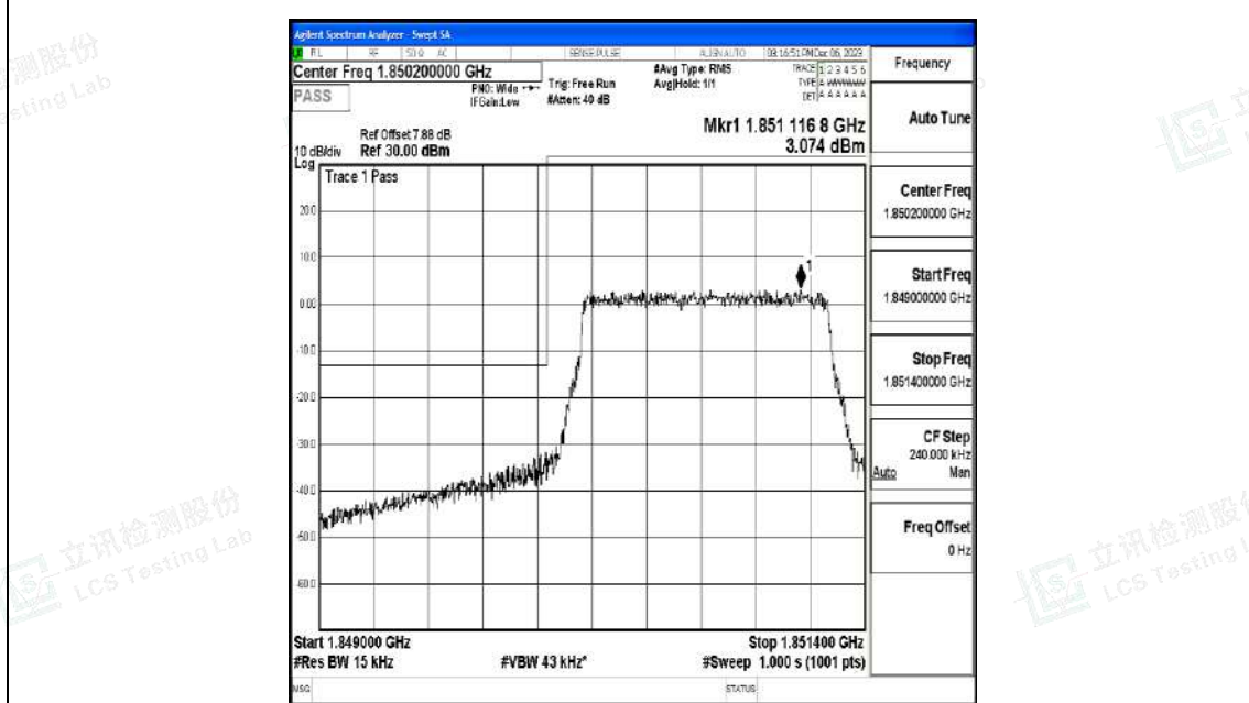
Band2_1.4MHz_16QAM_18607_6RB#0
