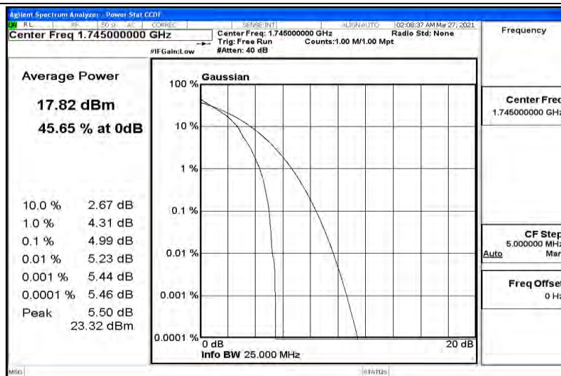
Band66-10MHz-QPSK-132322-50RB#0
