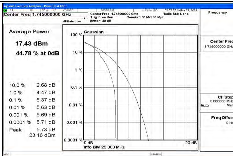
Band66-20MHz-QPSK-132322-100RB#0
