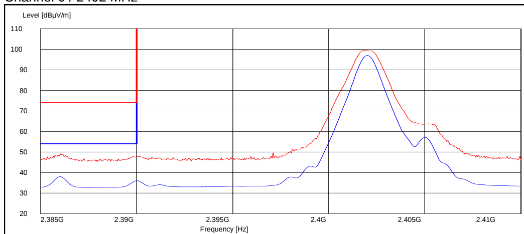
Channel 0 / 2402 MHz
