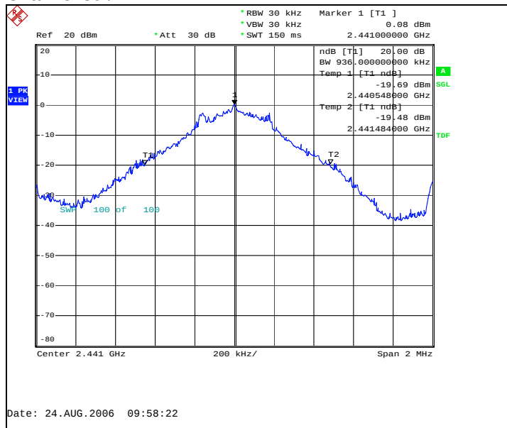
Channel 39 / 2441 MHz
