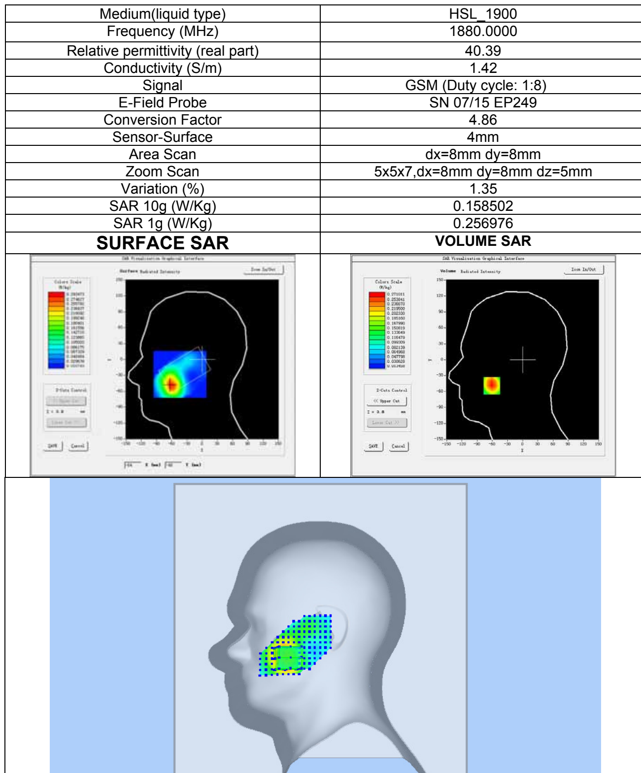
Plot 11: GSM1900, Middle channel (Right Head, Tilt) Product Description: MOBILE PHONE Test Date: Apr 14,2017
