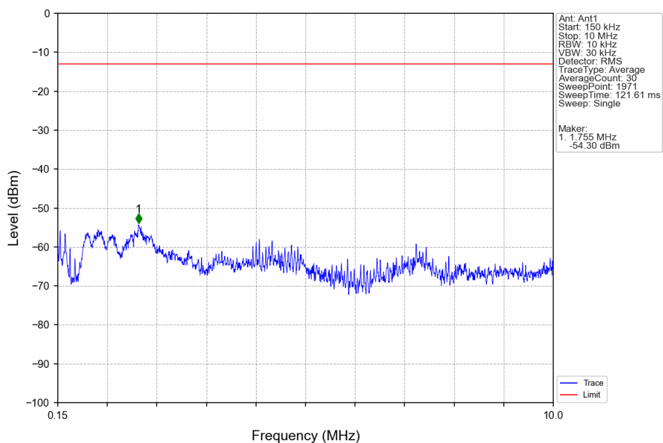
Band4_15MHz_16QAM_LCH_1717.5MHz_RB_1_0_NTNV
