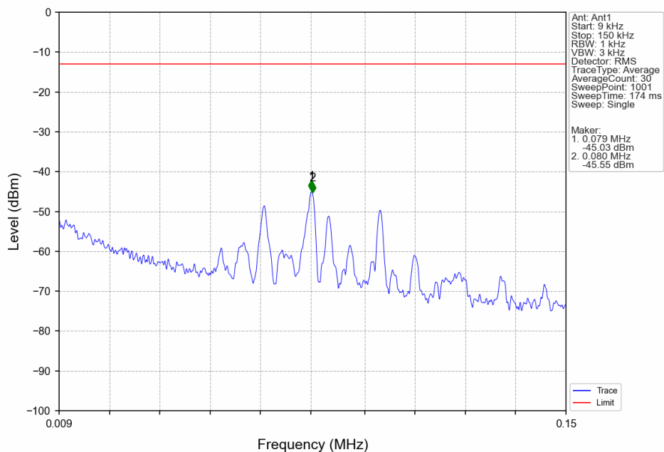
Band4 5MHz 16QAM HCH 1752.5MHz RB 1 0 NTNV
