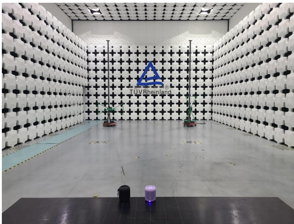
Photograph 2: Set-up photo for Radiated Emission, Below 1GHz
