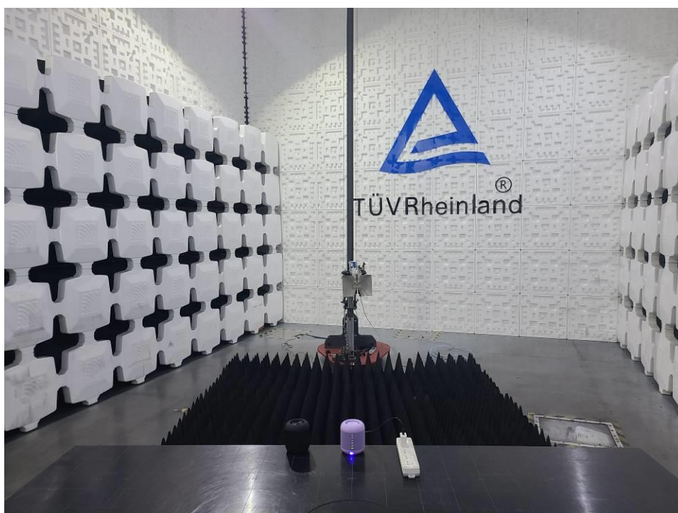
Photograph 3: Set-up photo for Radiated Emission, Above 1GHz
