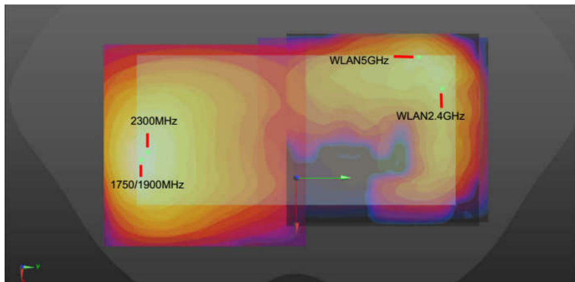
WWAN+WLAN2.4GHz/WWAN+WLAN5GHz_Back 0mm
