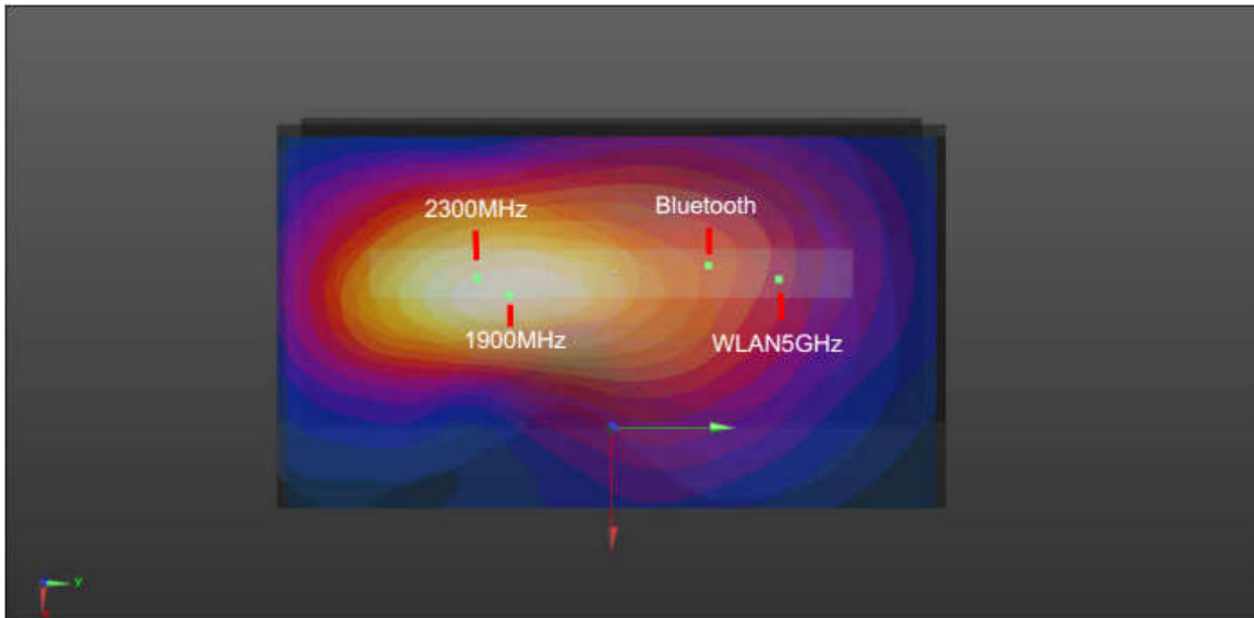
WWAN+WWAN5GHz+Bluetooth_Side 5mm
