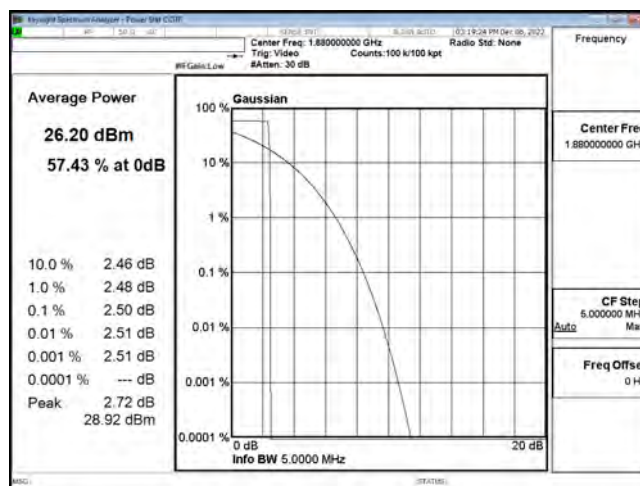
PTAR 2G1900 CH661 VOICE
