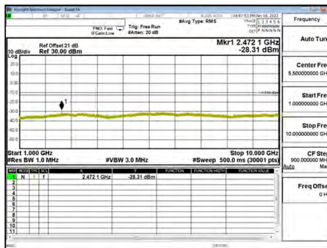
CSE 2G850 CH128 VOICE 1G-10G
