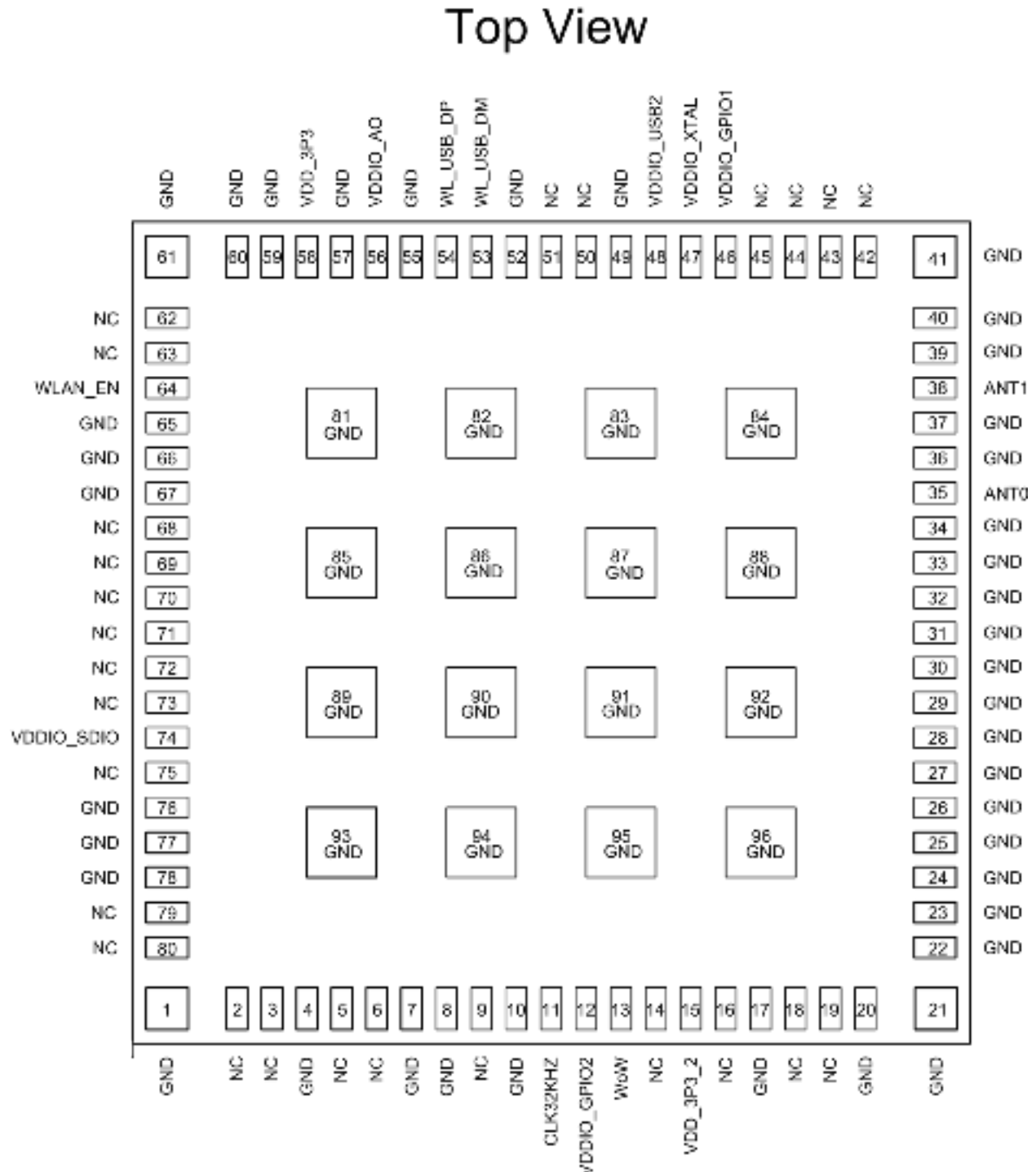
Figure 2: EVIA Module Pin Diagram
