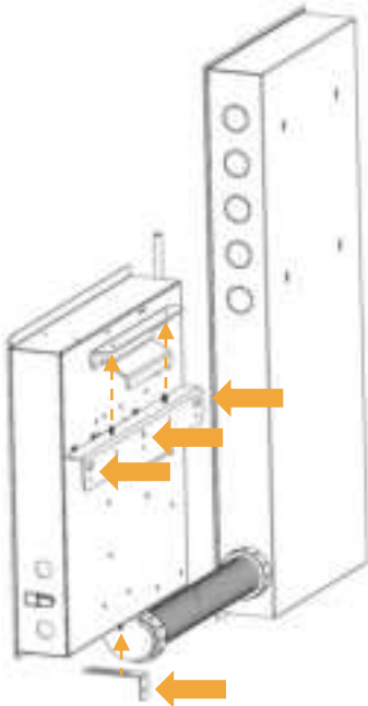
Location of Mounting Holes and Slots (Large Arrows) Bracket Attachment Stud Locations (Small Dashed Arrows)
