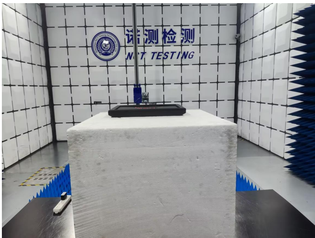
Setup Photo FCC ID: 2ABSC-7CL
