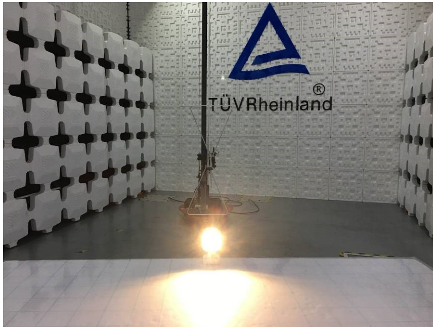
Photograph 3: Set-up for Radiated Emission, Below 1GHz
