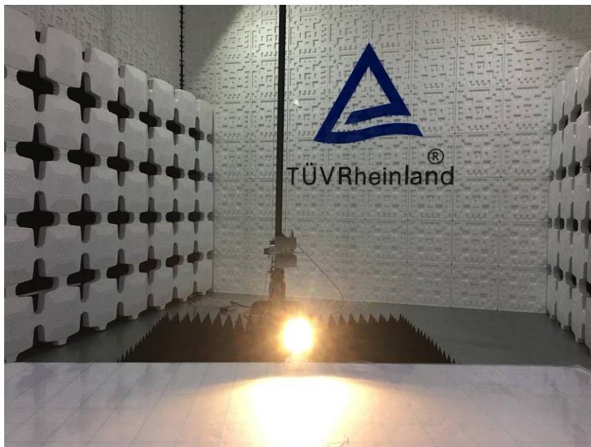
Photograph 4: Set-up for Radiated Emission, Above 1GHz
