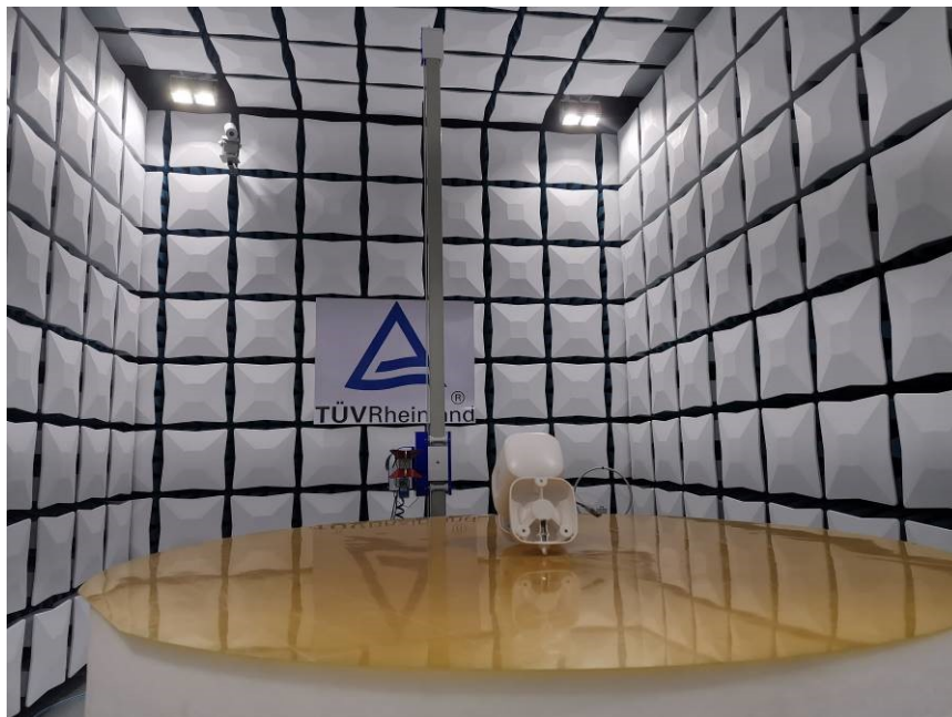
Photograph 2: Set-up for Radiated Spurious Emission, Above 1GHz
