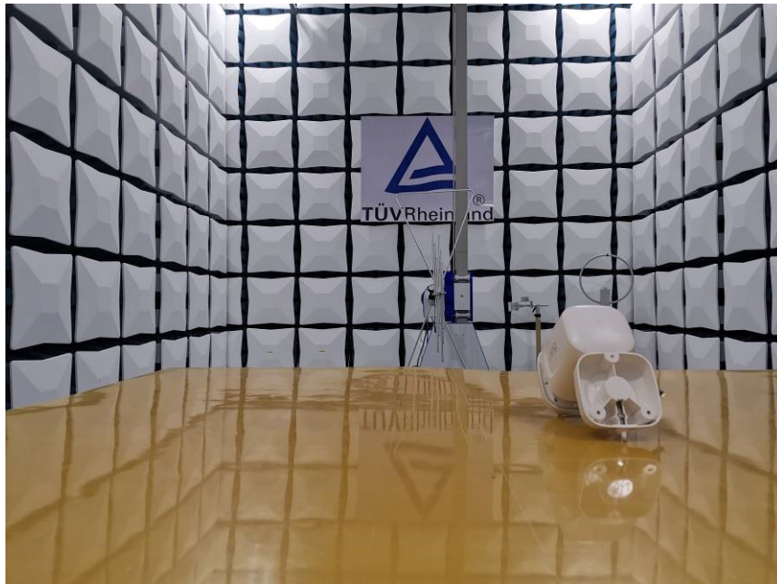
Photograph 1: Set-up for Radiated Spurious Emission, 30MHz ~ 1GHz
