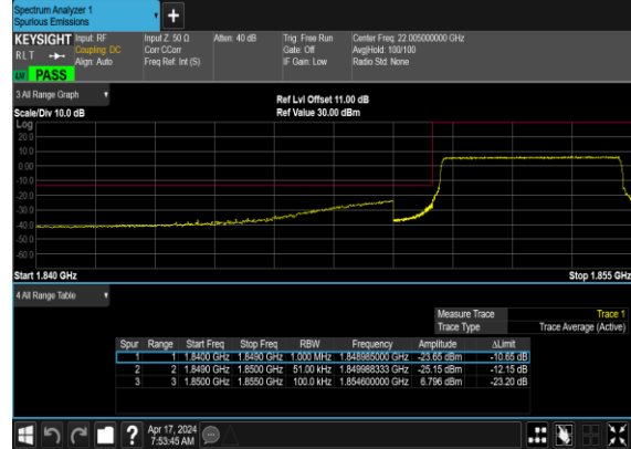
N25(5M)_CP- OFDM_QPSK_Outer_Full_Low_CH
