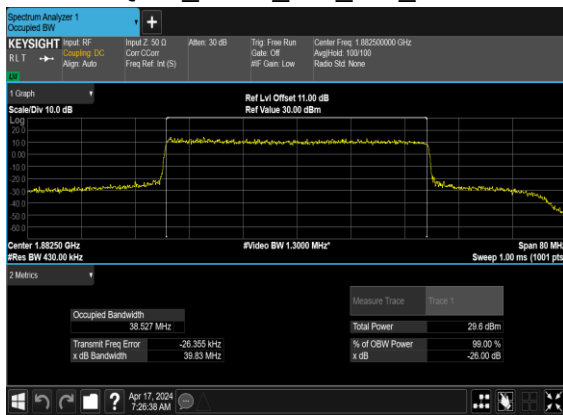
N25(40M)_CP-OFDM_16 QAM_Outer_Full_Mid_CH
