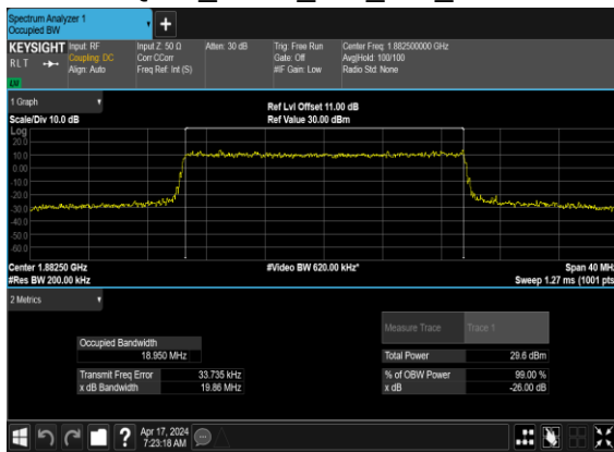
N25(20M)_CP-OFDM_16 QAM_Outer_Full_Mid_CH
