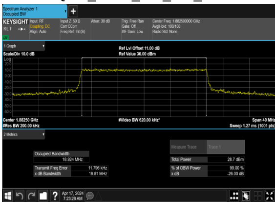
N25(20M)_CP-OFDM_64 QAM_Outer_Full_Mid_CH
