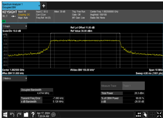
N25(5M)_CP-OFDM_64 QAM_Outer_Full_Mid_CH
