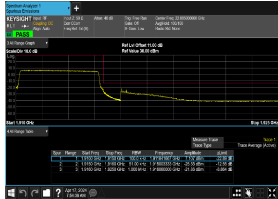
N25(5M)_CP- OFDM_QPSK_Outer_Full_High_CH
