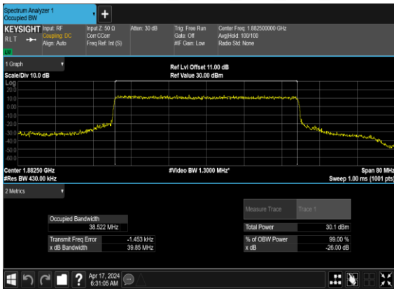
N25(40M)_CP- OFDM_QPSK_Outer_Full_Mid_CH
