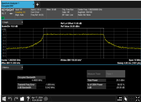
N25(5M)_CP-OFDM_QPSK_Outer_Full_Mid_CH
