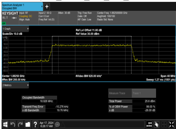
N25(20M)_CP-OFDM_256 QAM_Outer_Full_Mid_CH
