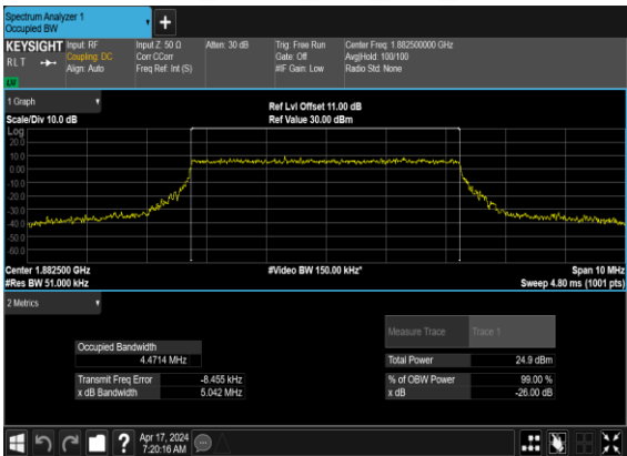
N25(5M)_CP-OFDM_256 QAM_Outer_Full_Mid_CH
