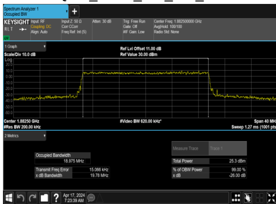
N25(20M)_CP-OFDM_256 QAM_Outer_Full_Mid_CH
