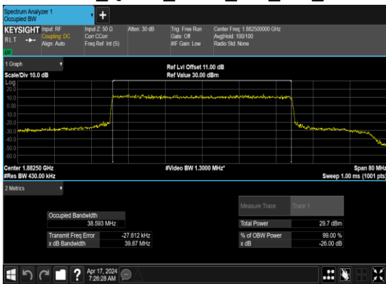
N25(40M)_CP- OFDM_QPSK_Outer_Full_Mid_CH
