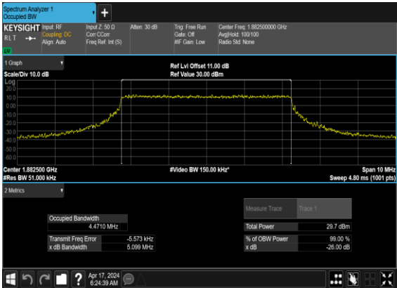
N25(5M)_CP-OFDM_16 QAM_Outer_Full_Mid_CH
