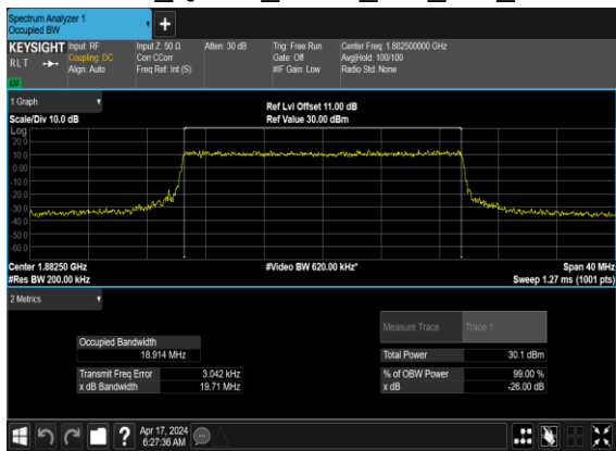
N25(20M)_CP- OFDM_QPSK_Outer_Full_Mid_CH
