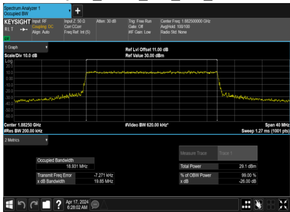
N25(20M)_CP-OFDM_64 QAM_Outer_Full_Mid_CH
