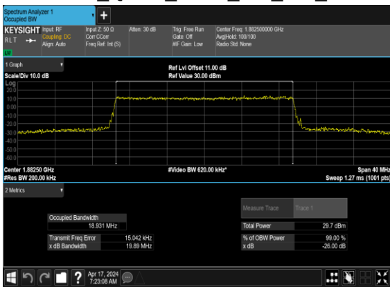
N25(20M)_CP- OFDM_QPSK_Outer_Full_Mid_CH
