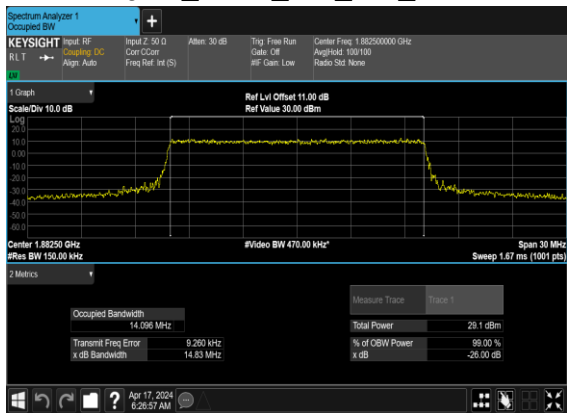
N25(15M)_CP-OFDM_64 QAM_Outer_Full_Mid_CH
