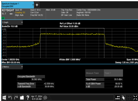
N25(40M)_CP-OFDM_16 QAM_Outer_Full_Mid_CH
