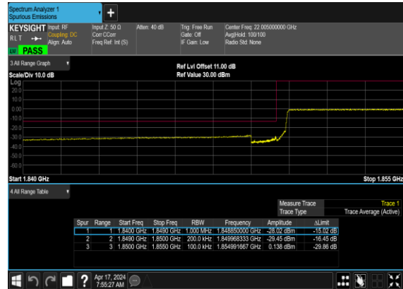
N25(20M)_CP- OFDM_QPSK_Outer_Full_Low_CH
