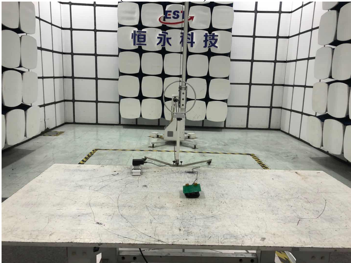
Radiated Test (9kHz-30 MHz)
