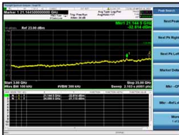
8-DPSK MIDDLE CHANNEL, SPURIOUS 3 GHz ~ 25 GHz
