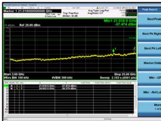
8-DPSK HIGH CHANNEL, SPURIOUS 3 GHz ~ 25 GHz
