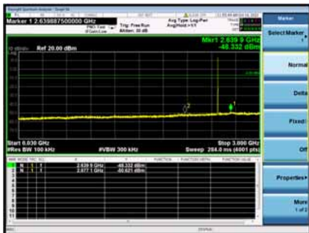
8-DPSK HIGH CHANNEL, SPURIOUS 30 MHz ~ 3 GHz
