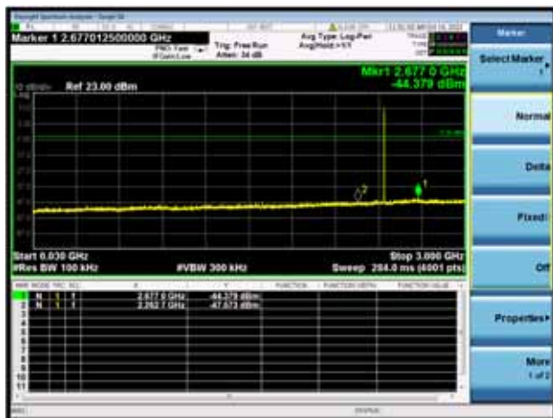
8-DPSK MIDDLE CHANNEL, SPURIOUS 30 MHz ~ 3 GHz
