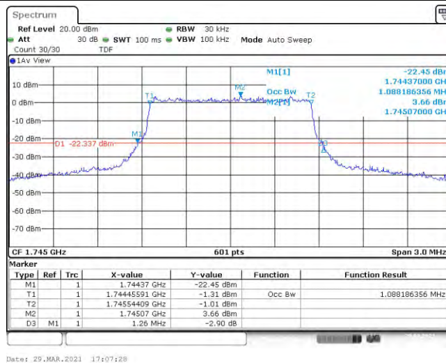
Band66-1.4MHz-16QAM-132665-6RB#0-1.088
