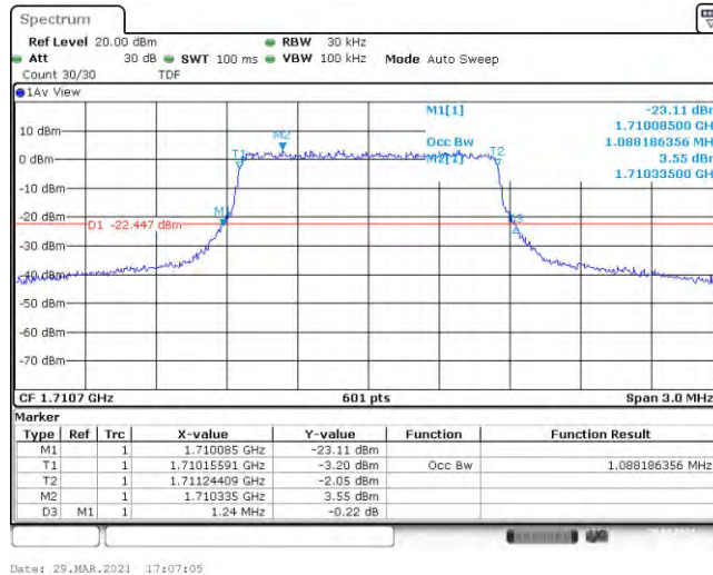
Band66-1.4MHz-16QAM-132322-6RB#0-1.088
