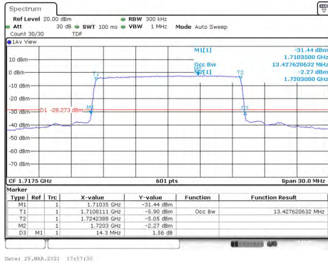
Band66-15MHz-16QAM-132322-75RB#0-13.428
