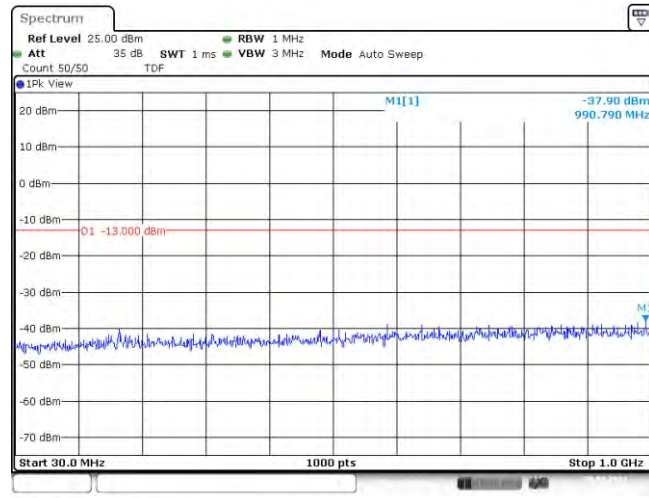
Band66-1.4MHz-QPSK-131979-1RB#0-Range1:30~1000MHz
