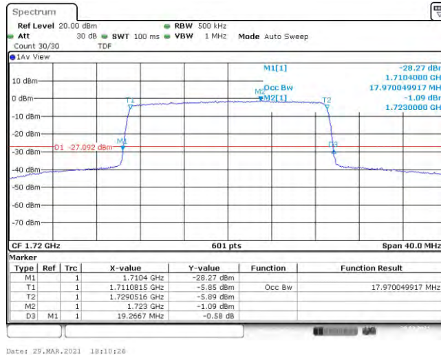
Band66-20MHz-16QAM-132322-100RB#0-17.97
