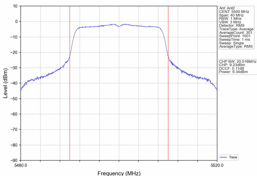
802.11ac(VHT20)_LCH_5500MHz_Ant2_NTNV
