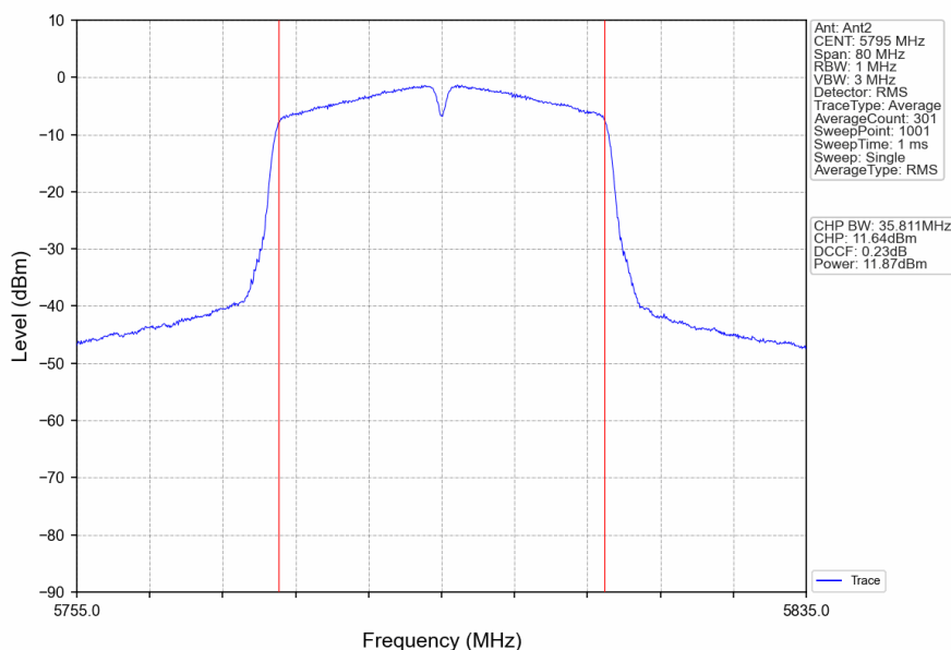
802.11ac(VHT40)_HCH_5795MHz_Ant2_NTNV
