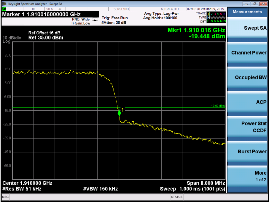
WCDMA band II band edge-right side
