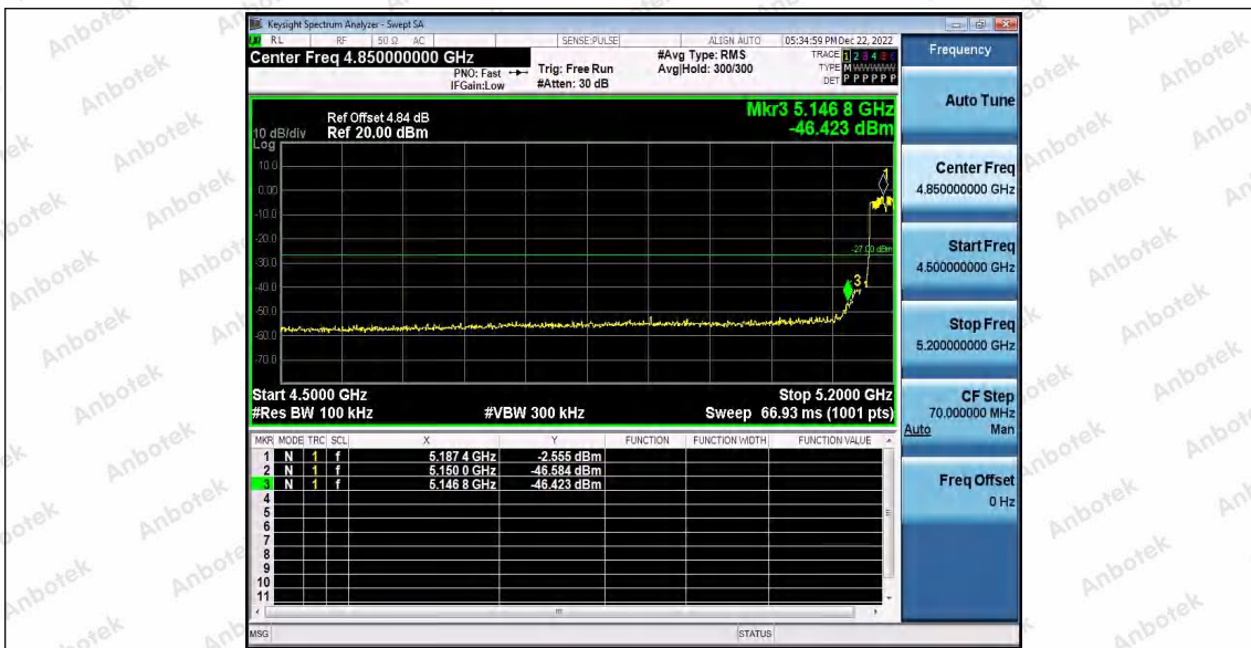
11AC40SISO_Ant2_Low_5190
