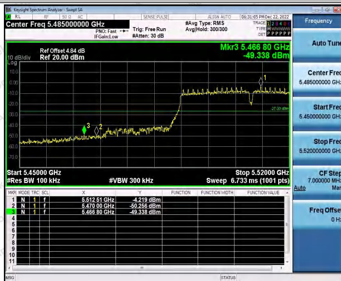
11AC40SISO_Ant2_Low_5510
