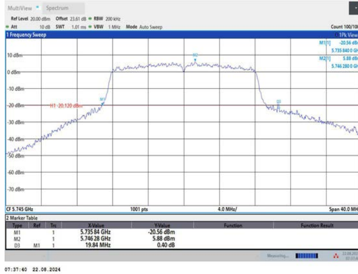
11A_Ant3_5745
