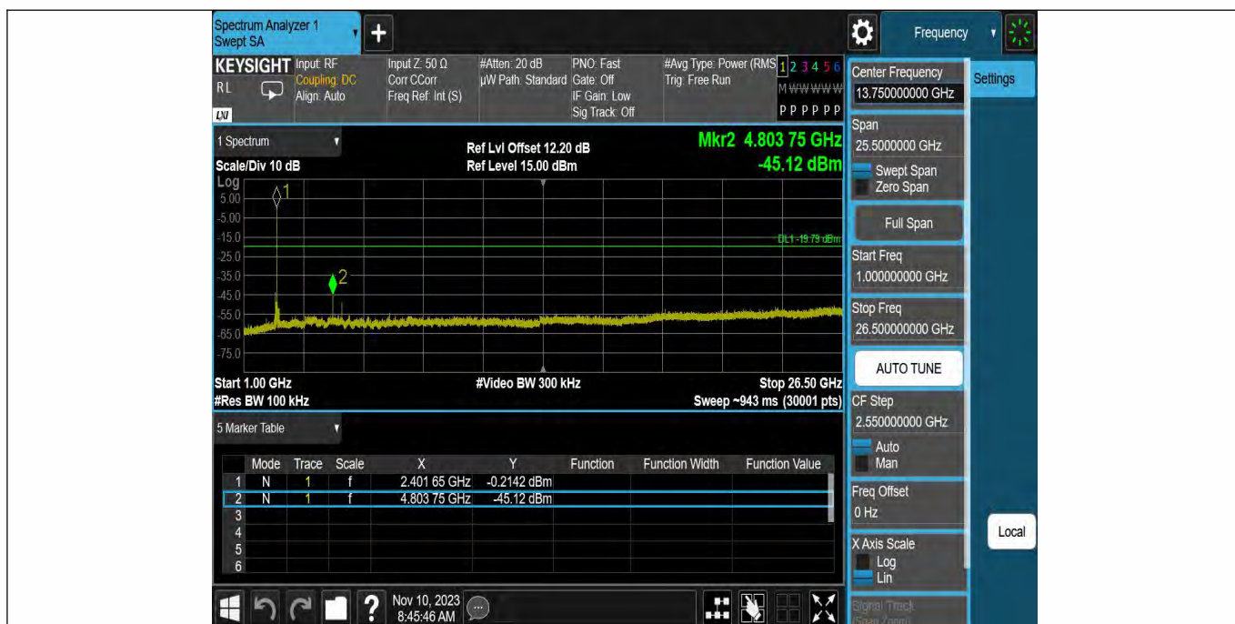
DH5-Ant1-2402-1000~26500
