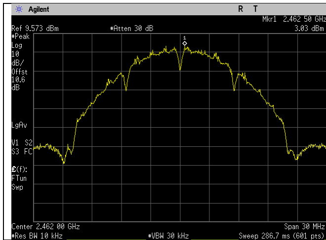
2462MHz_b-mode
