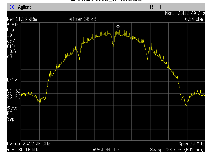
2412MHz_b-mode
