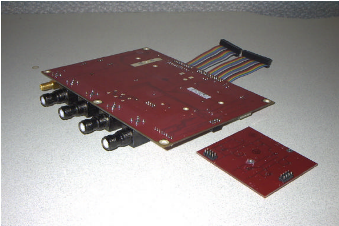
ALR 9800 RF board Bottom View Disassembled
