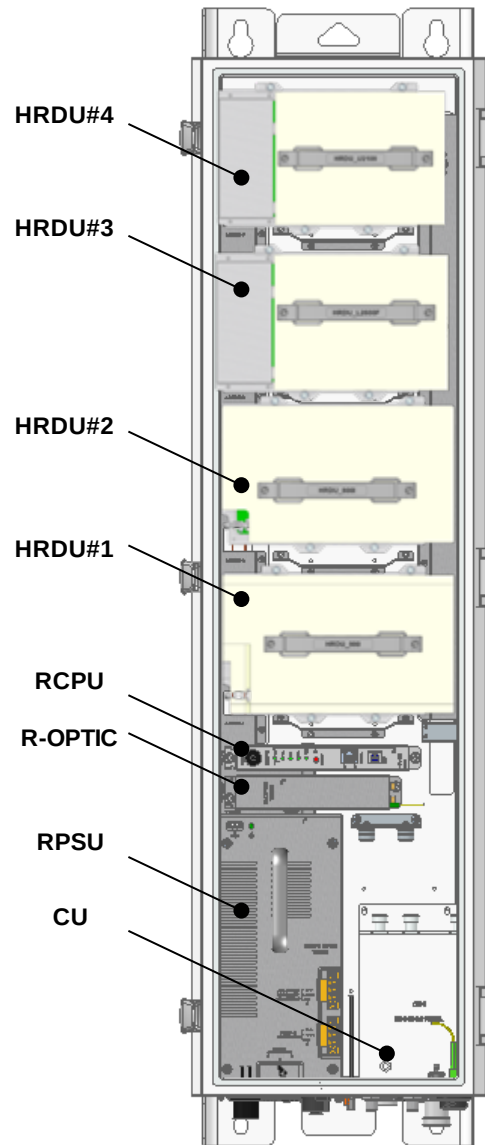
Figure 5. Inside of Remote Unit
