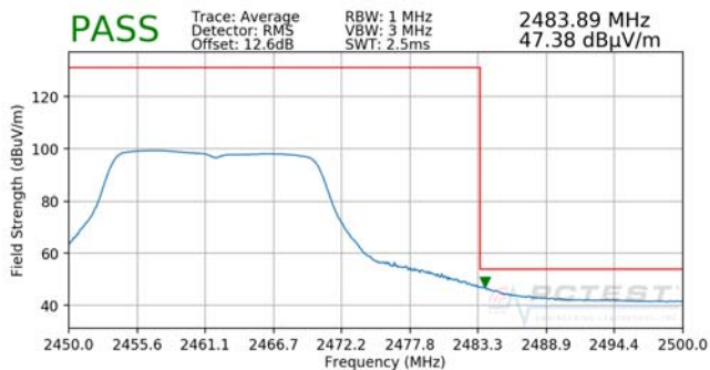
Plot 7-37. Radiated Restricted Upper Band Edge Measurement (Average)
