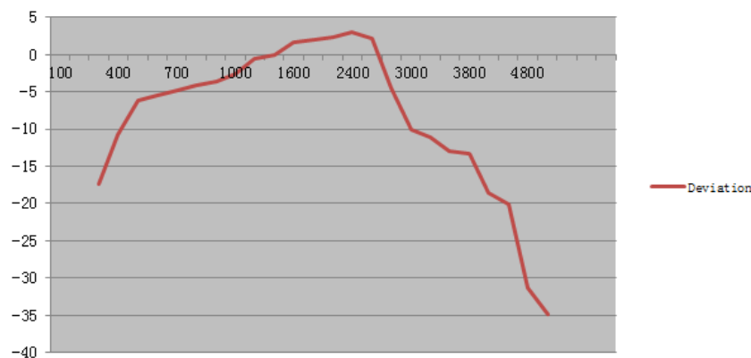
Audio Frequency Response@50%MI 10 KHz Channel Separations
