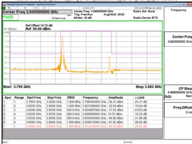
Band77-Part27_30MHz_CP_OFDM_SCS30kHz_OPSK_RB1_0_CH656000
