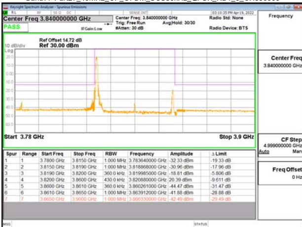
Band77-Part27_40MHz_CP_OFDM_SCS30kHz_QPSK_RB1_0_CH656000
