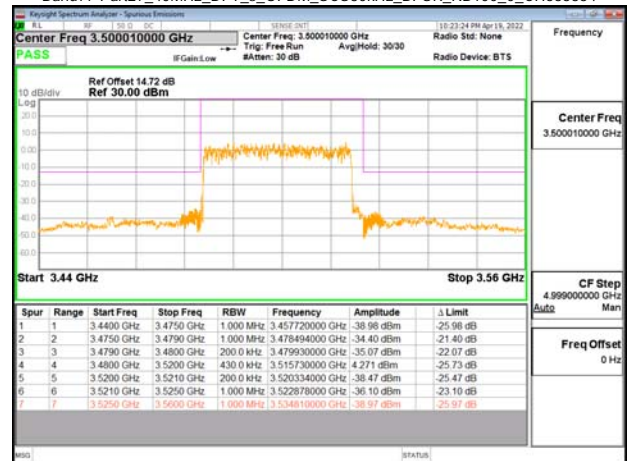
Band77-Part27_40MHz_DFT_s_OFDM_SCS30kHz_BPSK_RB100_0_CH633334
