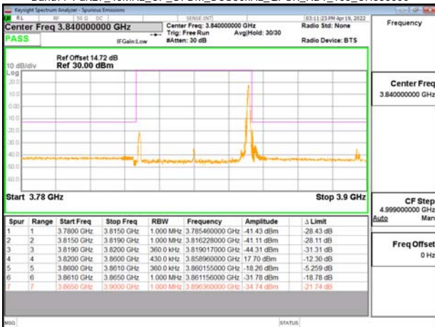
Band77-Part27_40MHz_CP_OFDM_SCS30kHz_OPSK_RB1_105_CH656000
