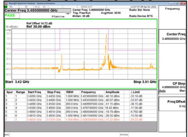
Band77-Part27_30MHz_CP_OFDM_SCS30kHz_OPSK_RB1_77_CH633334
