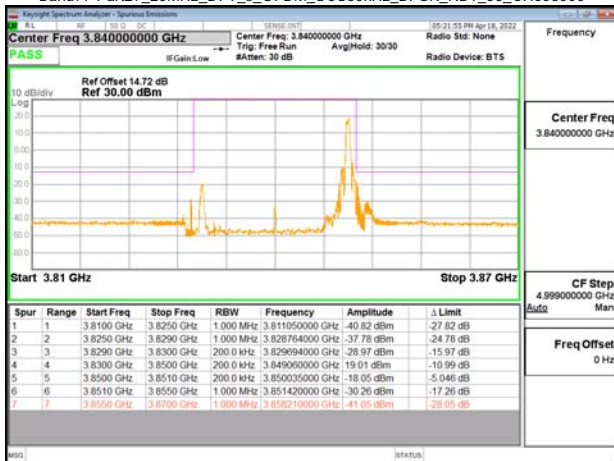
Band77-Part27_20MHz_DFT_s_OFDM_SCS30kHz_BPSK_RB1_50_CH656000
