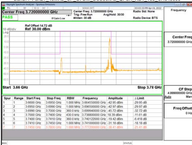
Band77-Part27_40MHz_CP_OFDM_SCS30kHz_OPSK_RB1_105_CH656000
