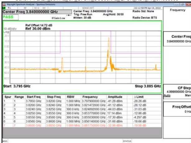
Band77-Part27_30MHz_CP_OFDM_SCS30kHz_QPSK_RB1_77_CH656000
