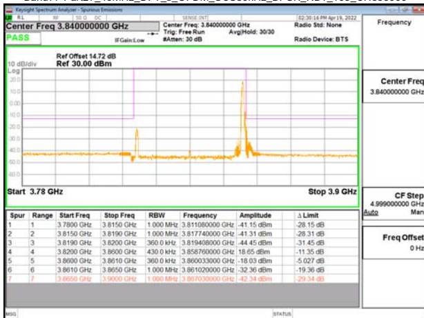
Band77-Part27_40MHz_DFT_s_OFDM_SCS30kHz_BPSK_RB1_105_CH656000
