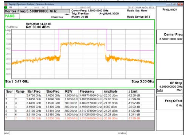
Band77-Part27_20MHz_CP_OFDM_SCS30kHz_QPSK_RB51_0_CH633334
