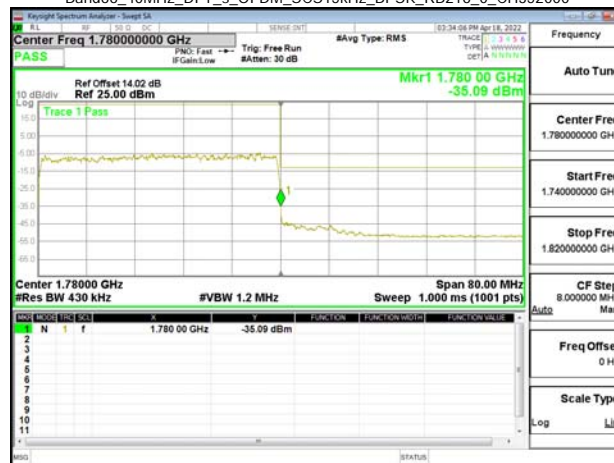
Band66_40MHz_DFT_s_OFDM_SCS15kHz_BPSK_RB216_0_CH352000
