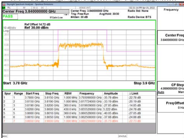
Band77-Part27_40MHz_DFT_s_OFDM_SCS30kHz_BPSK_RB100_0_CH656000
