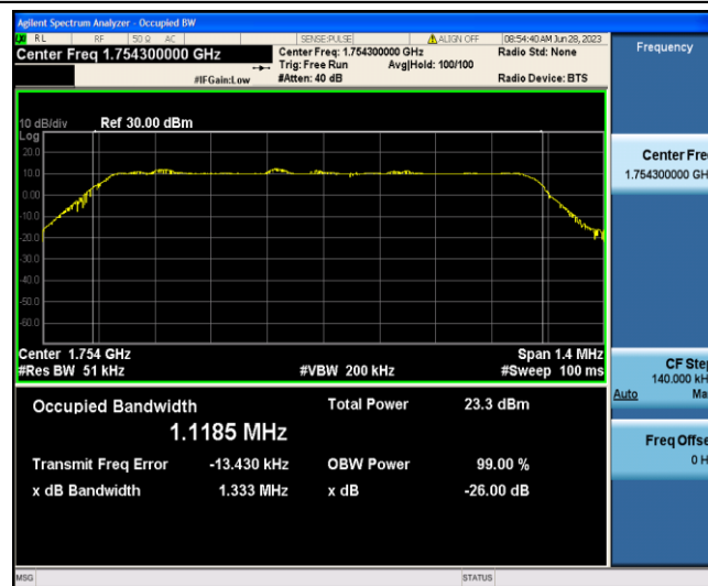
Band4-1.4MHz-QPSK-20393-6-0-Low-1.1185-1.333-PASS
