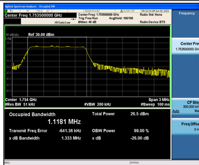
Band4-3MHz-16QAM-20385-6-0-Low-1.1181-1.333-PASS
