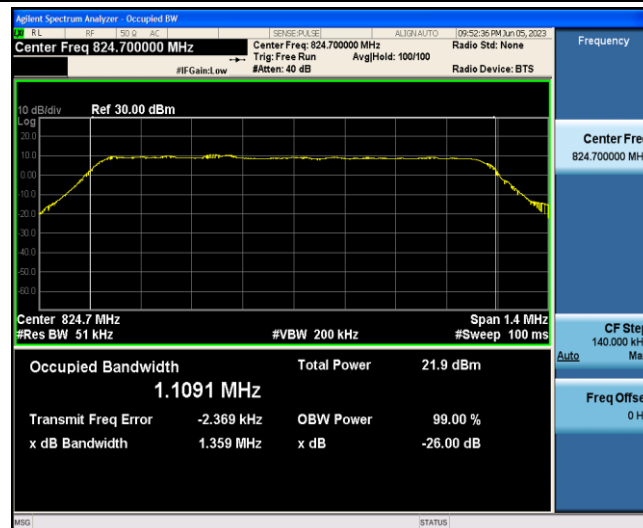
Band5-1.4MHz-QPSK-20407-6-0-Low-1.1091-1.359-PASS
