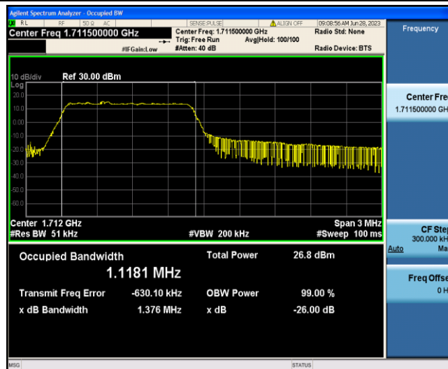
Band4-3MHz-QPSK-19965-6-0-Low-1.1181-1.376-PASS
