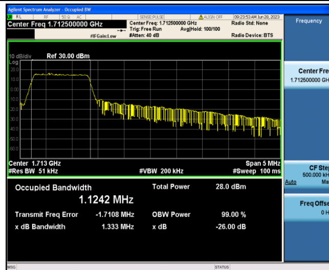
Band4-5MHz-QPSK-19975-6-0-Low-1.1242-1.333-PASS
