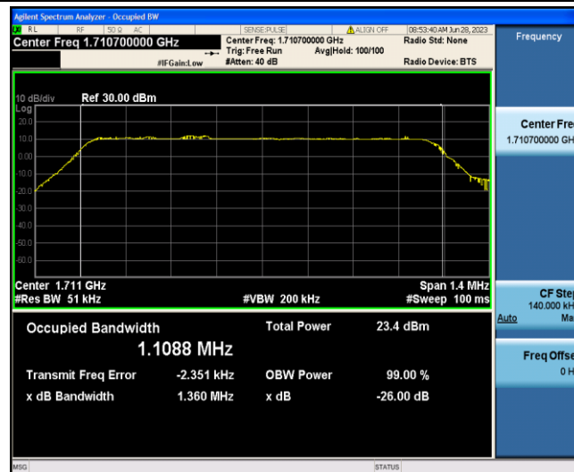
Band4-1.4MHz-16QAM-19957-6-0-Low-1.1088-1.360-PASS
