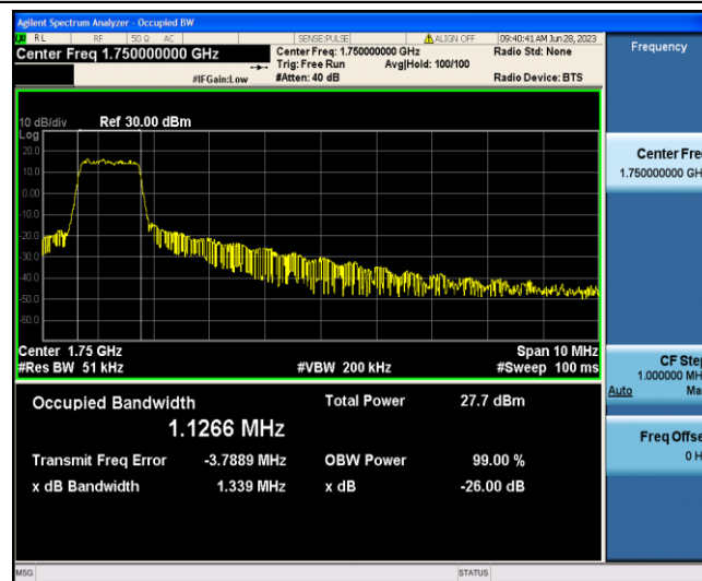
Band4-10MHz-16QAM-20350-6-0-Low-1.1266-1.339-PASS
