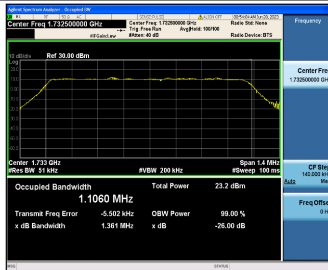
Band4-1.4MHz-QPSK-20175-6-0-Low-1.1060-1.361-PASS
