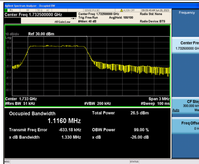
Band4-3MHz-16QAM-20175-6-0-Low-1.1160-1.330-PASS
