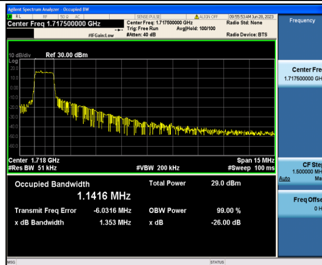
Band4-15MHz-QPSK-20025-6-0-Low-1.1416-1.353-PASS
