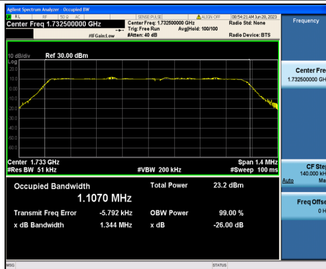
Band4-1.4MHz-16QAM-20175-6-0-Low-1.1070-1.344-PASS
