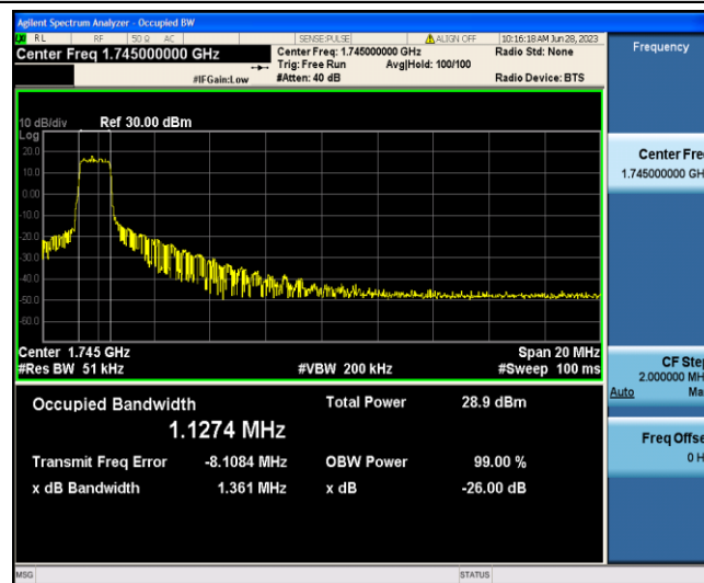
Band4-20MHz-16QAM-20300-6-0-Low-1.1274-1.361-PASS
