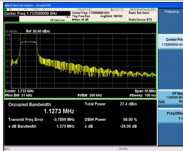
Band4-10MHz-16QAM-20175-6-0-Low-1.1273-1.375-PASS
