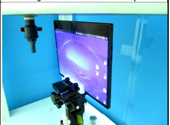
Bottom Side of EUT with 15 mm Gap
