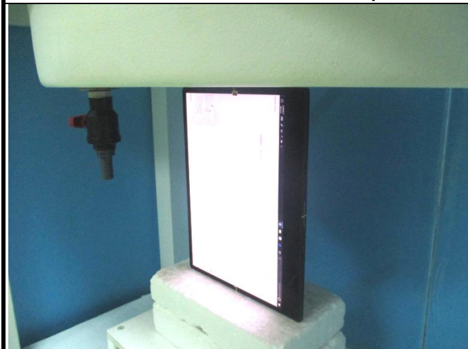
Right Side of EUT with 0 mm Gap
