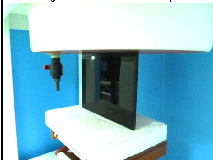
Bottom Side of EUT with 0 mm Gap
