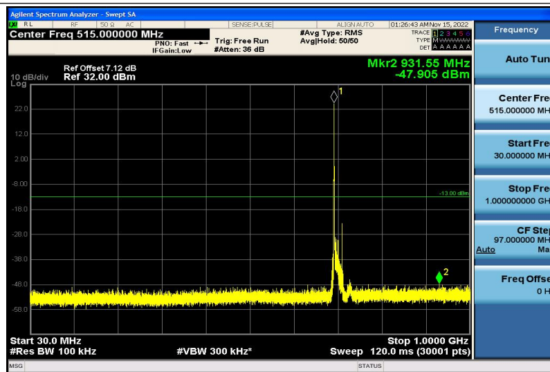
Band12-10MHz-16QAM-23060-1RB#0-30~1000MHz
