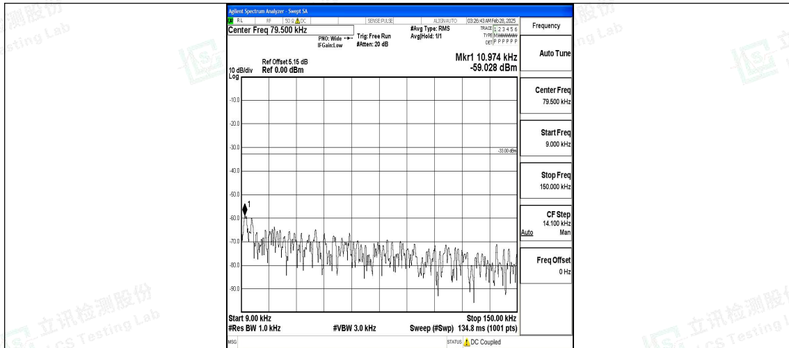
Band12_1.4MHz_16QAM_23095_1RB#0_0.009~0.15_0.009~0.15
