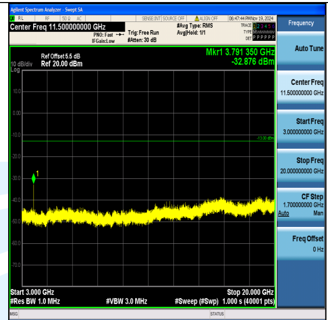
Band2_15MHz_16QAM_19125_1RB#0_3000~20000_3000~20000
