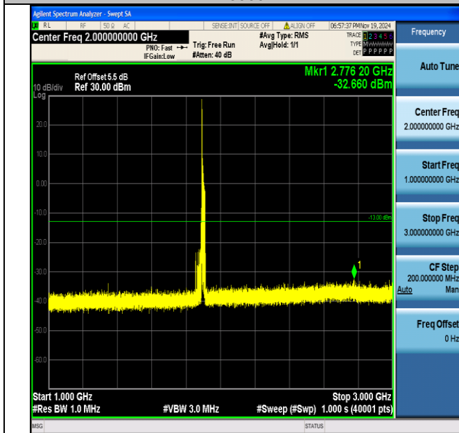
Band2_20MHz_16QAM_19100_1RB#0_1000~3000_1000~3000
