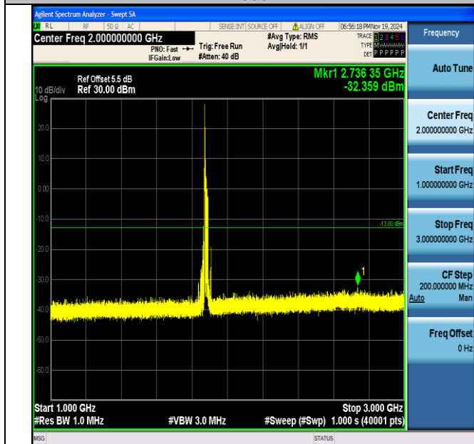
Band2_20MHz_QPSK_18900_1RB#0_1000~3000_1000~3000
