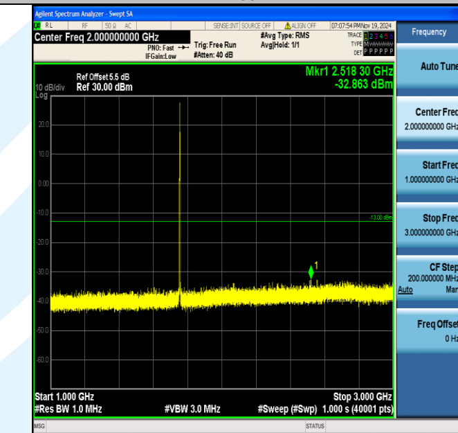
Band4_1.4MHz_QPSK_20393_1RB#0_1000~3000_1000~3000
