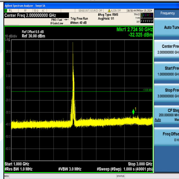
Band2_20MHz_16QAM_18900_1RB#0_1000~3000_1000~3000
