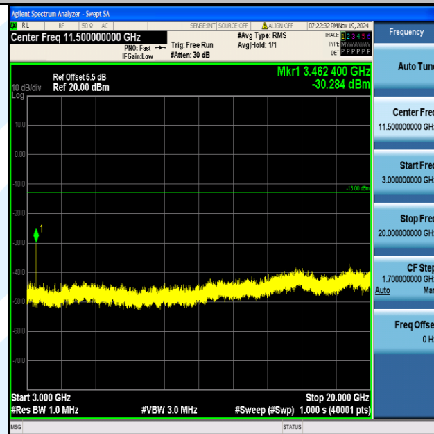
Band4_3MHz_QPSK_20175_1RB#0_3000~20000_3000~20000
