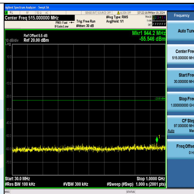
Band4_3MHz_QPSK_20175_1RB#0_30~1000_30~1000
