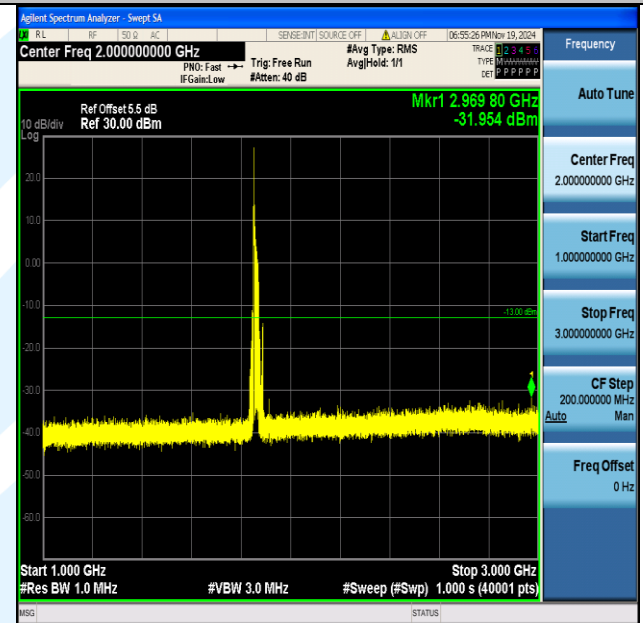
Band2_20MHz_QPSK_18700_1RB#0_1000~3000_1000~3000
