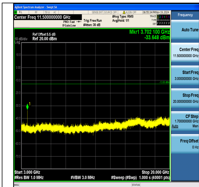
Band2_20MHz_QPSK_18700_1RB#0_3000~20000_3000~20000
