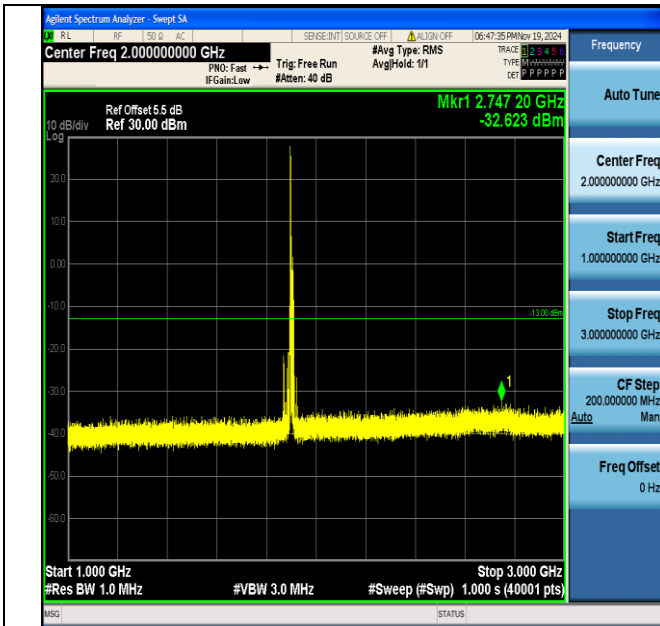
Band2_15MHz_16QAM_19125_1RB#0_1000~3000_1000~3000
