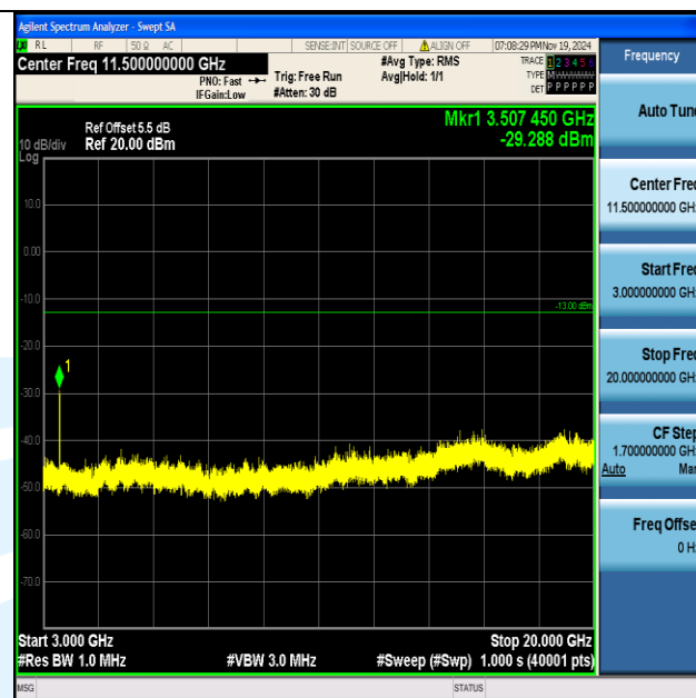
Band4_1.4MHz_16QAM_20393_1RB#0_3000~20000_3000~20000
