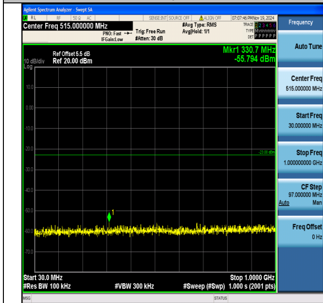
Band4_1.4MHz_QPSK_20393_1RB#0_30~1000_30~1000
