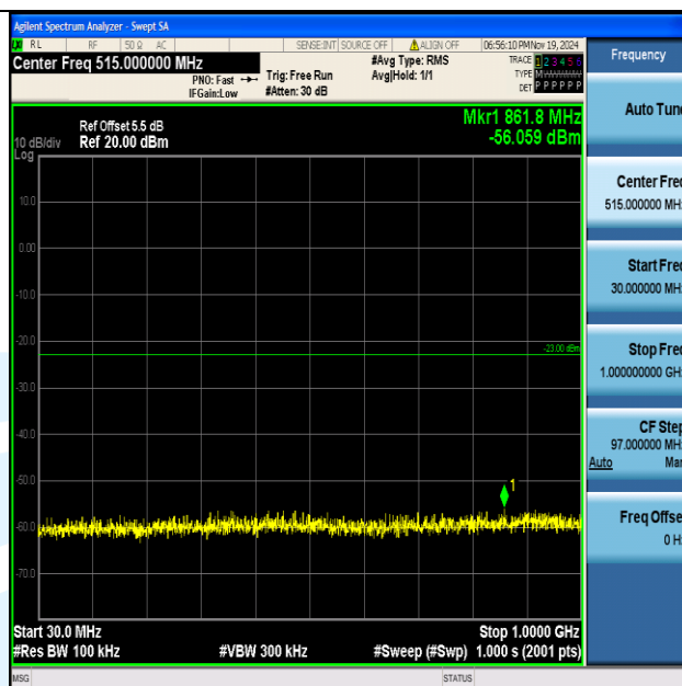
Band2_20MHz_QPSK_18900_1RB#0_30~1000_30~1000
