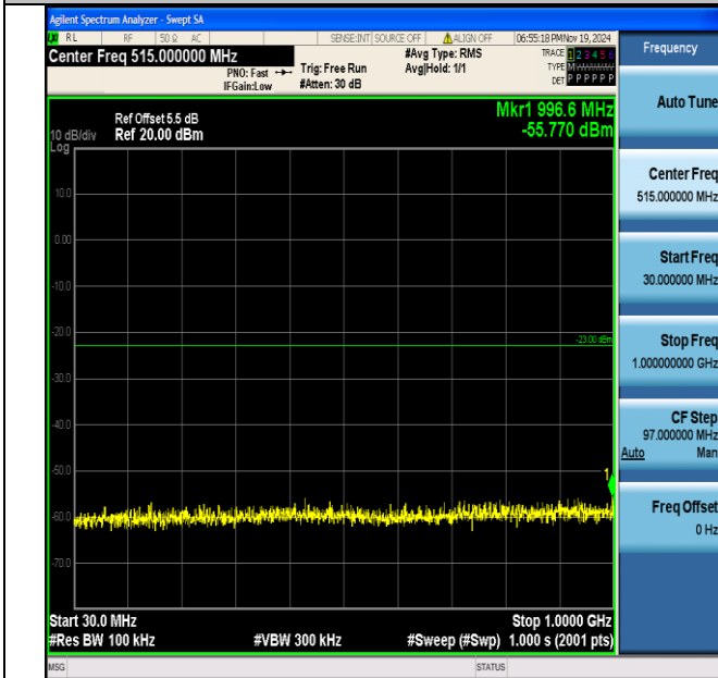
Band2_20MHz_QPSK_18700_1RB#0_30~1000_30~1000
