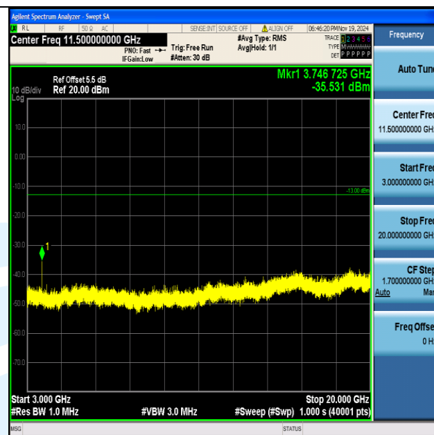
Band2_15MHz_QPSK_18900_1RB#0_3000~20000_3000~20000
