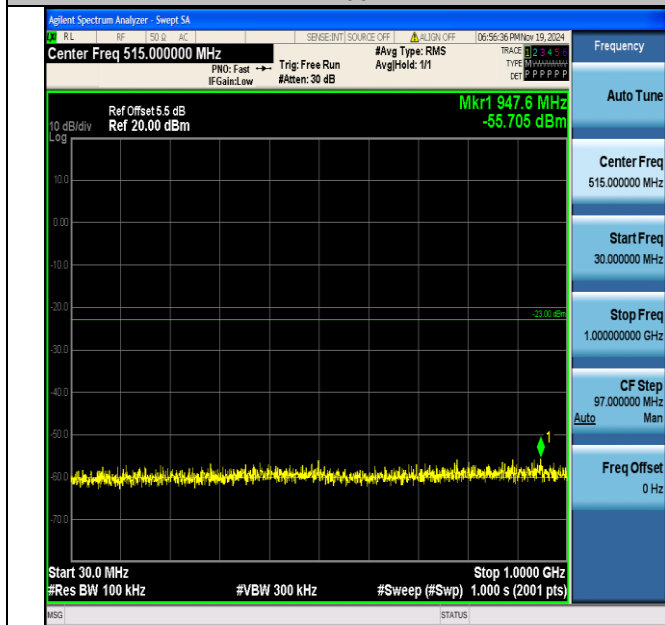
Band2_20MHz_16QAM_18900_1RB#0_30~1000_30~1000
