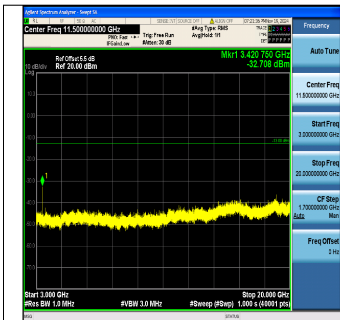
Band4_3MHz_QPSK_19965_1RB#0_3000~20000_3000~20000
