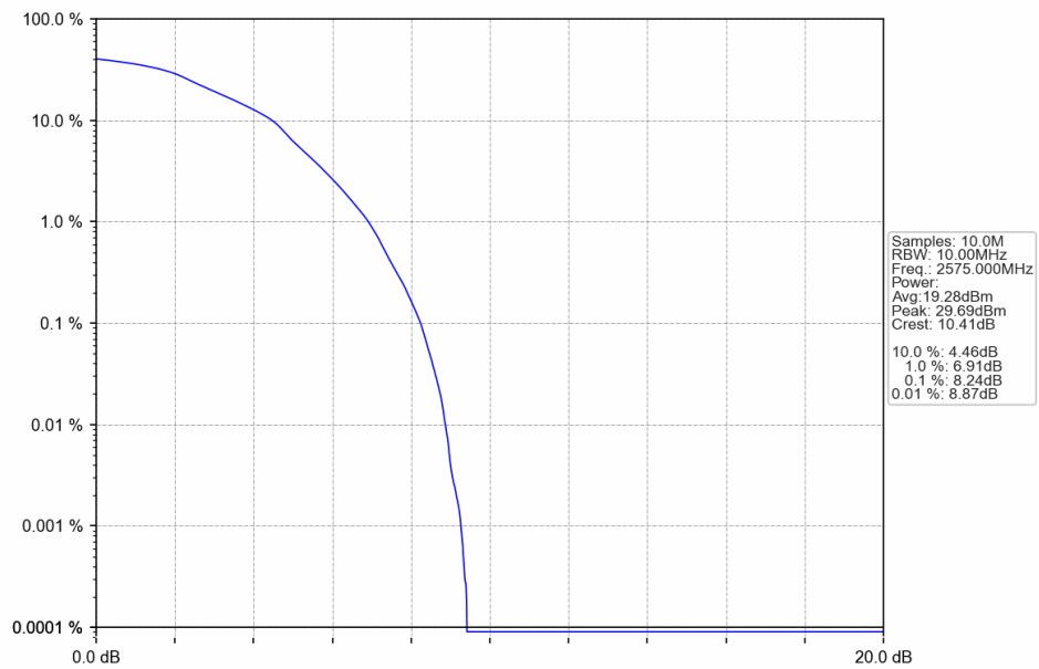
Band38 10MHz 16QAM LCH 2575MHz RB 27 0 NTNV
