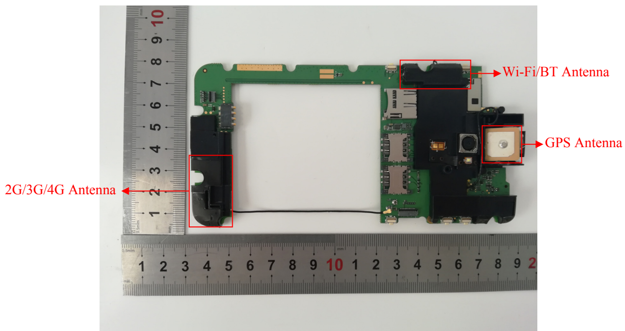
EUT – Cover off View-5
